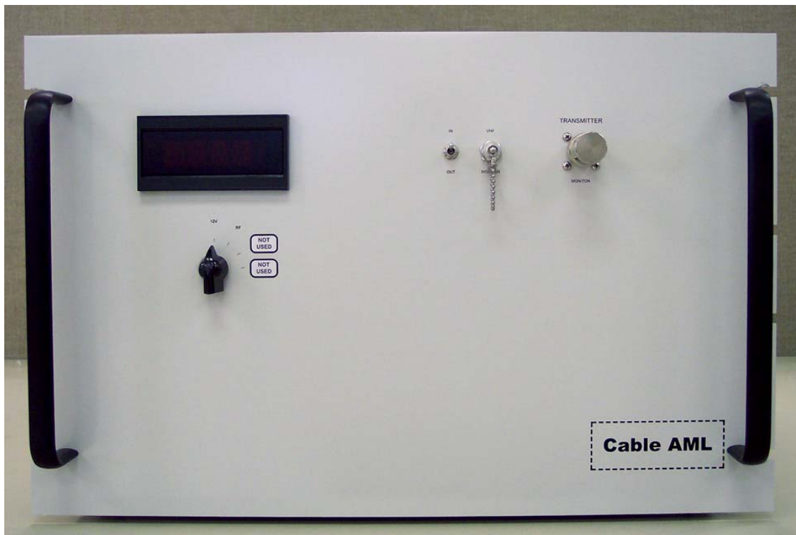
Figure 5. Front Panel Connection Points.
