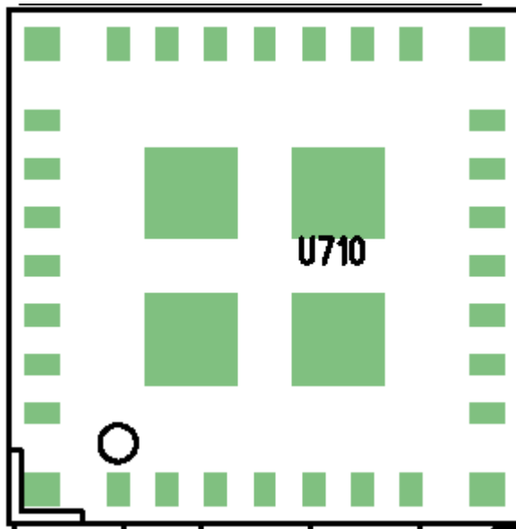
Fig.4-2. Top view of RF Transceiver PCB Layout
