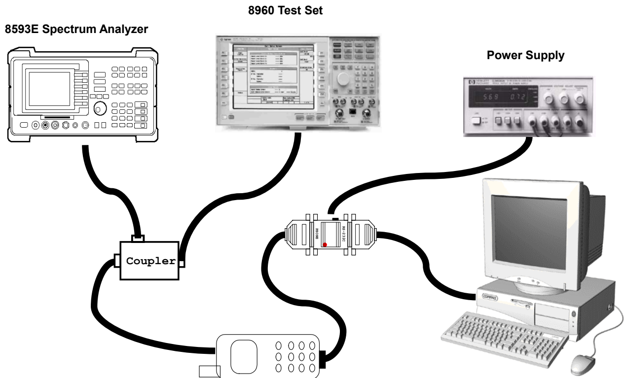
Fig.5-1. Test Set Configuration
