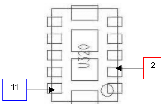
Fig. 6-11 U320 Antenna Switch Module PCB Layout
