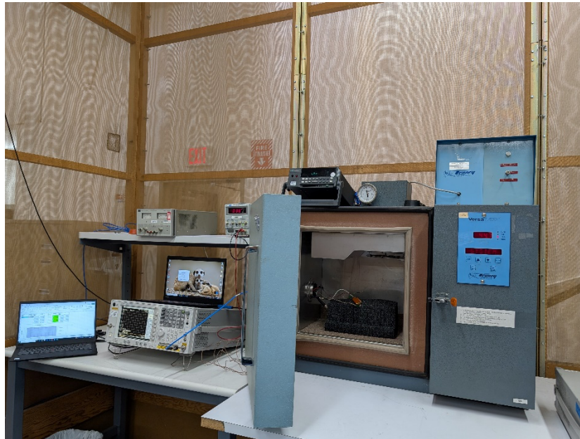
Frequency Stability 1
