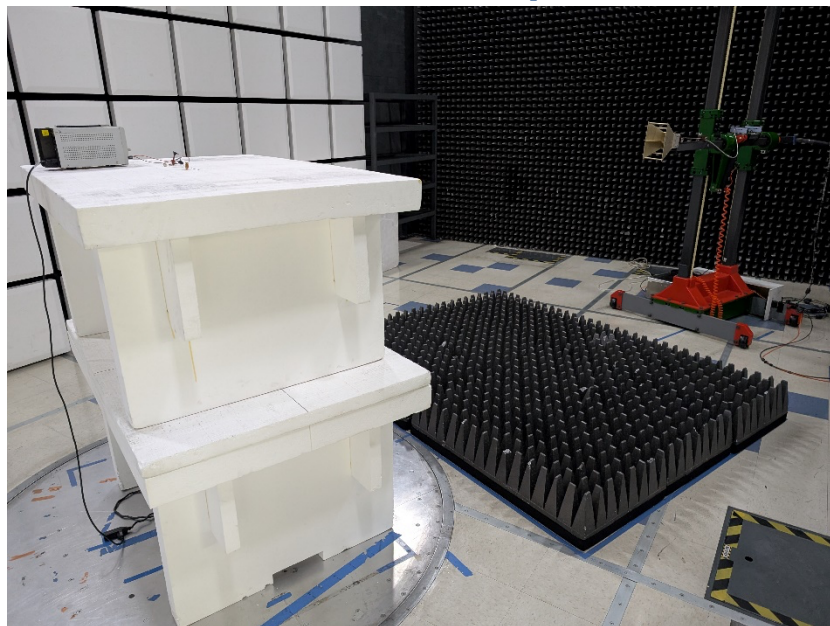
Above 1GHz Setup
