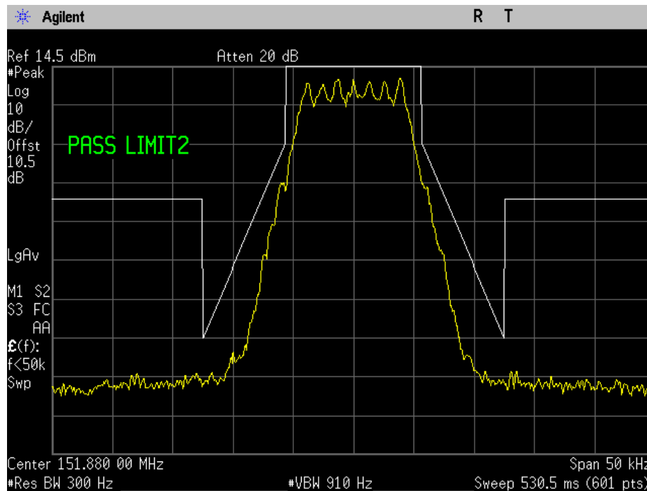
151.88 MHz Mask
