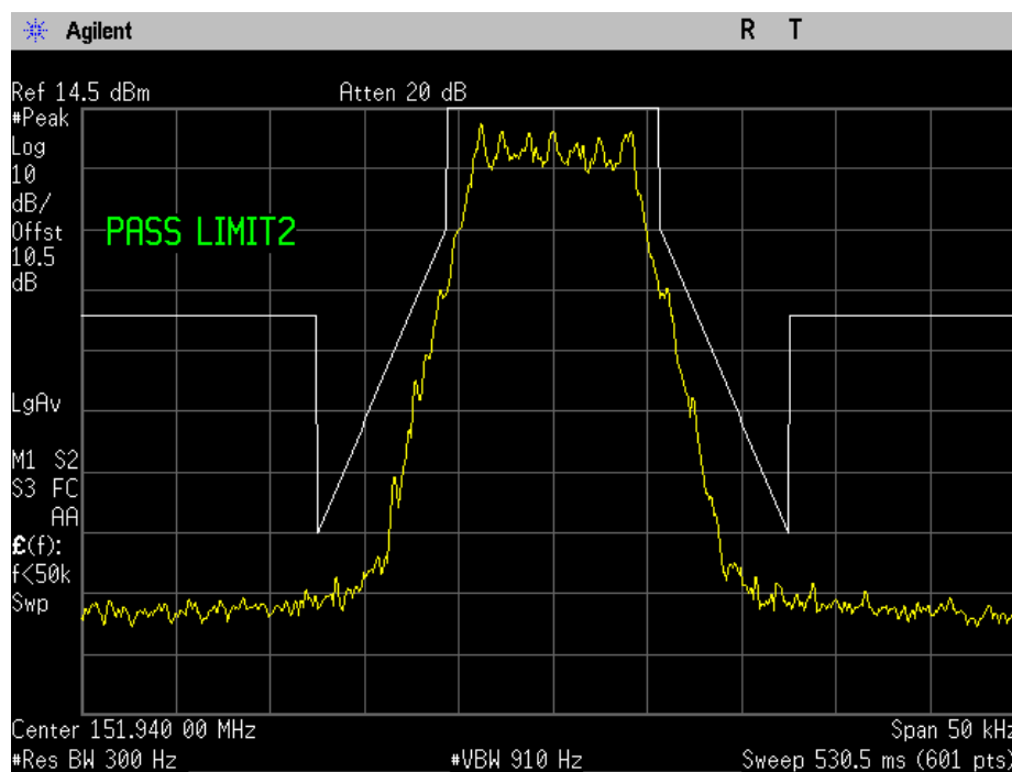
151.94 MHz Mask
