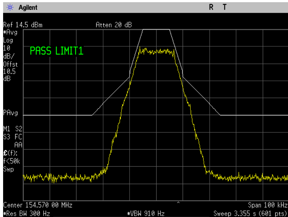
154.57 MHz Mask
