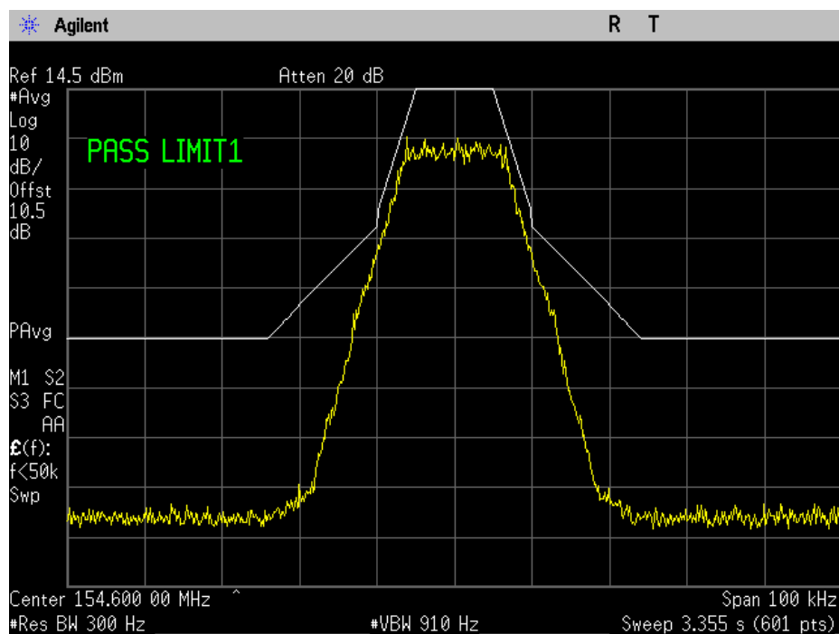
154.60 MHz Mask
