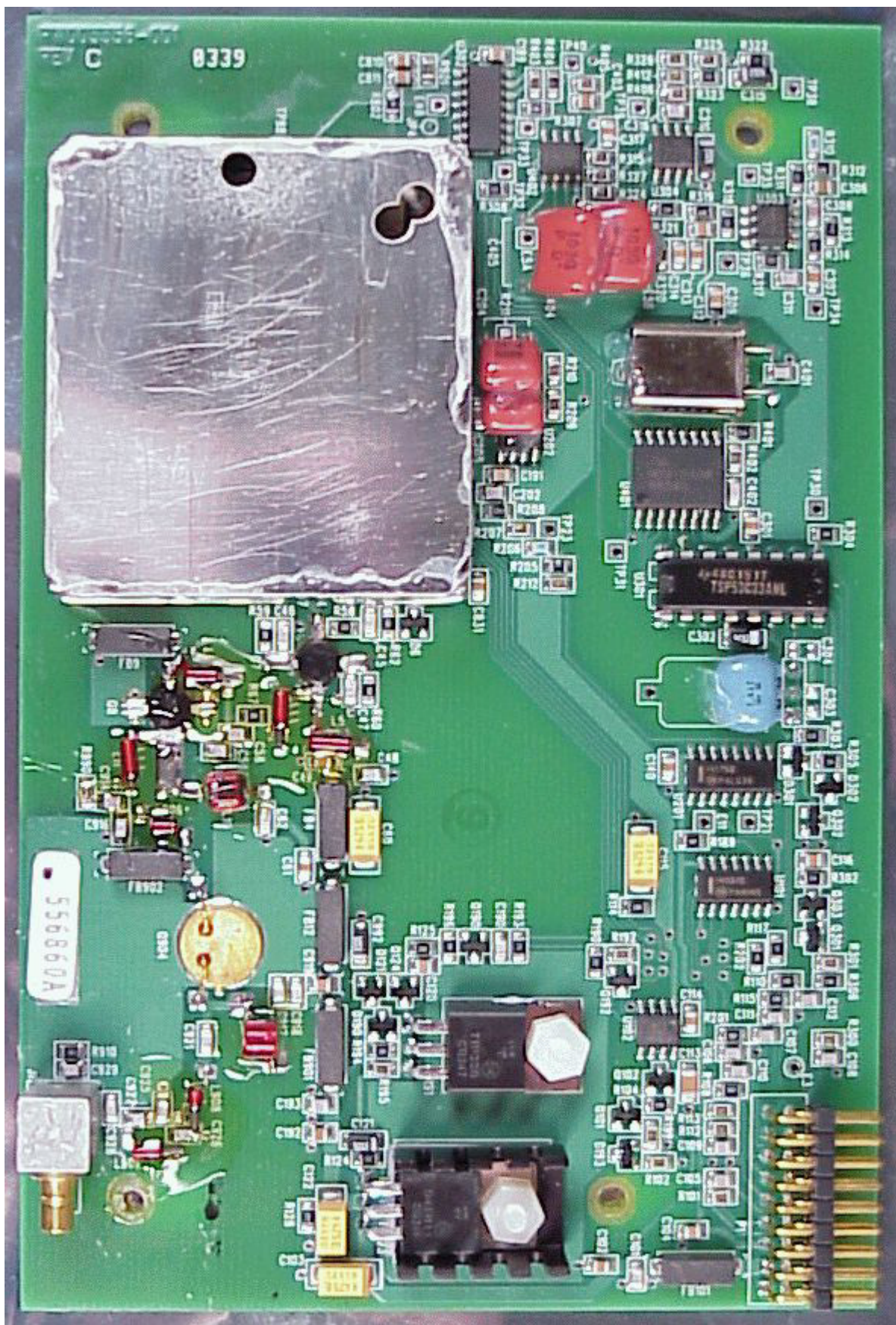
PT-200/PT-210/PT-210M Transmitter Board – Top Side
