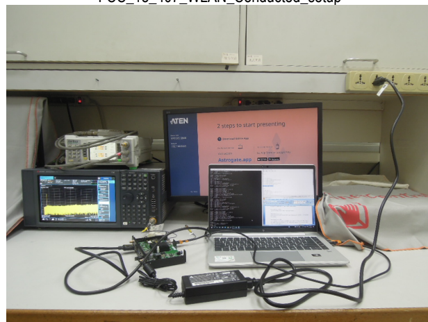
FCC_15_407_WLAN_Conducted_setup
