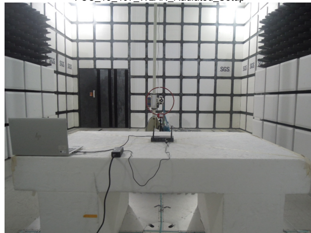
FCC_15_407_WLAN_Radiated_Setup
