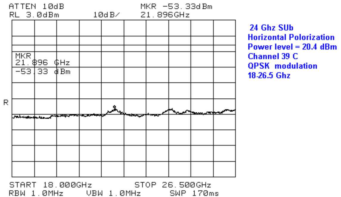
Figure 41 Radiated Emissions in 18-26.5GHz, HP, for transmitting 20dBm QPSK on Channel 39C
