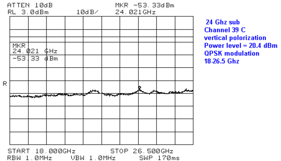
Figure 47 Radiated Emissions in 18-26.5GHz, VP, for transmitting 20dBm QPSK on Channel 39C
