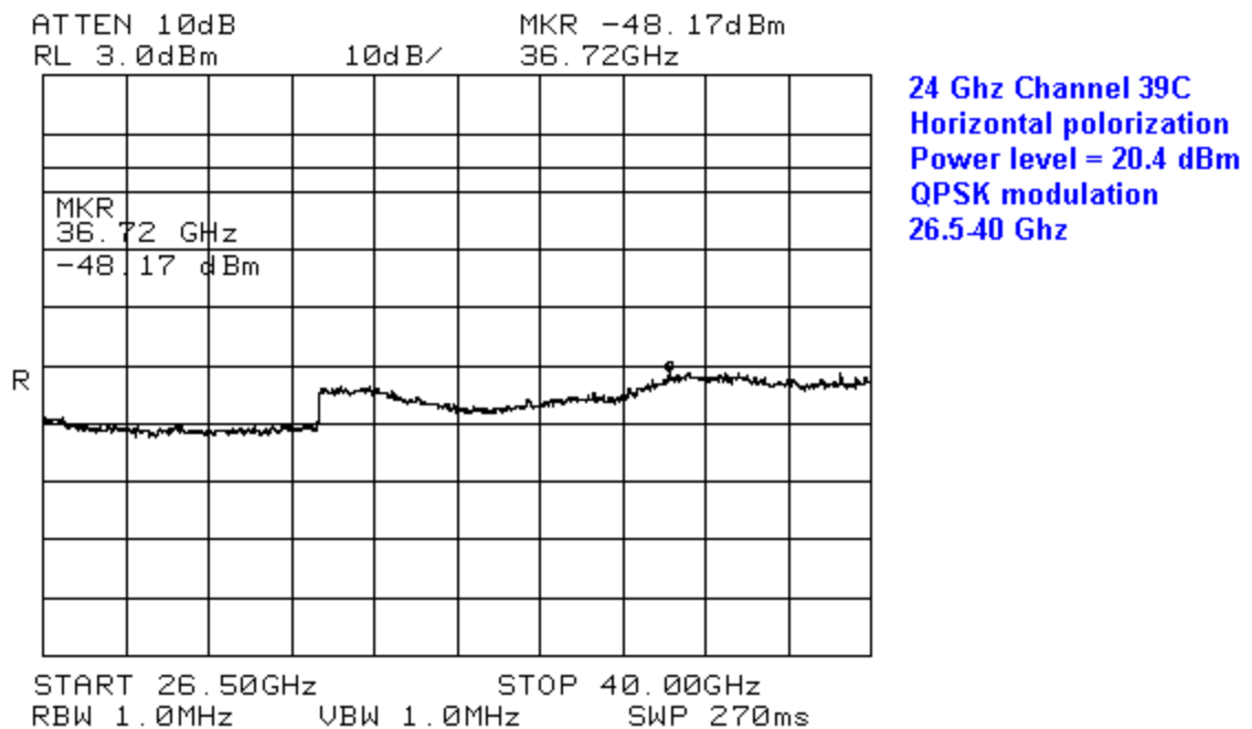
Figure 42 Radiated Emissions in 26.5-40GHz, HP, for transmitting 20dBm QPSK on Channel 39C
