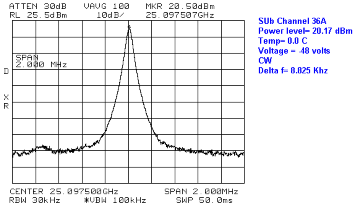
Figure60: T=0 °C -48VDC, Tx Power = 20.0 dBm
