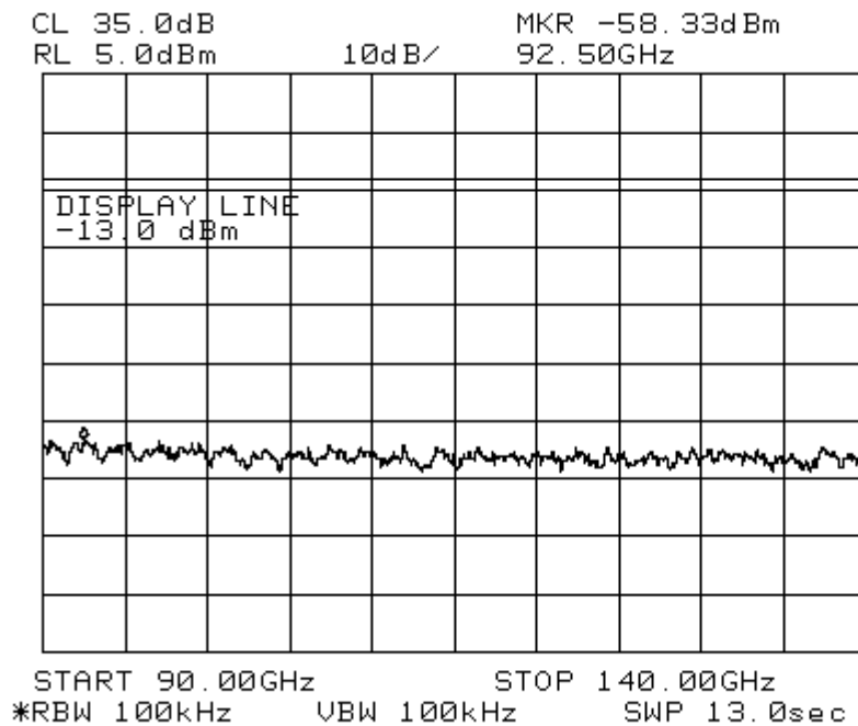
Figure 44 Conducted Emissions in 90 – 140 GHz, for transmitting -12 dBm on channel 7B4
