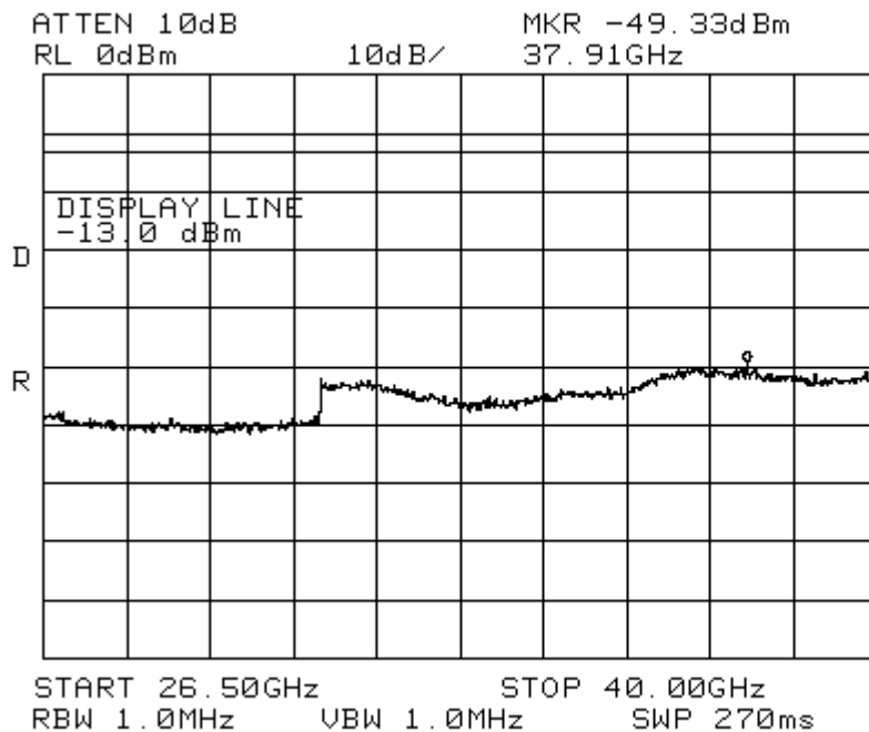
Figure 57 Radiated Emissions in 26.5 – 40 GHz, for transmitting 18 dBm on channel 4B3
