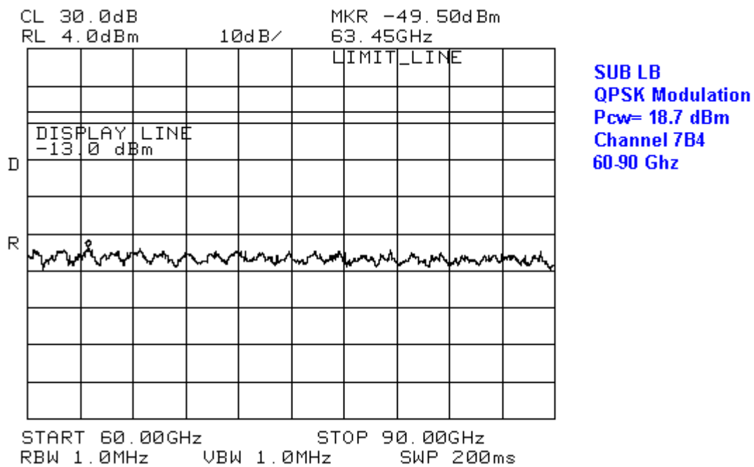
Figure 31 Conducted Emissions in 60 – 90 GHz, for transmitting 18 dBm on channel 7B4
