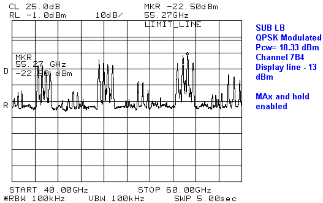
Figure 30 Conducted Emissions in 40 – 60 GHz, for transmitting 18 dBm on channel 7B4
