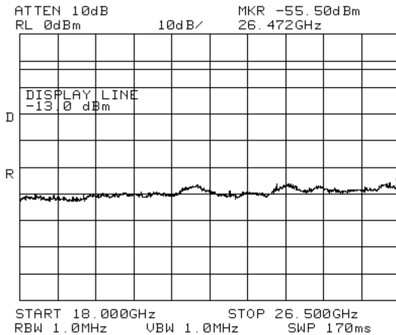
Figure 56 Radiated Emissions in 18 – 26.5 GHz, for transmitting 18 dBm on channel 4B3
