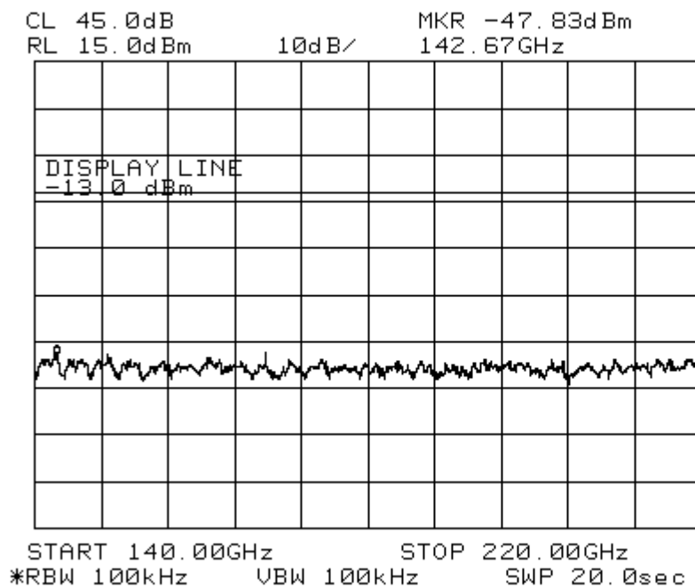
Figure 45 Conducted Emissions in 140 – 220 GHz, for transmitting -12 dBm on channel 7B4
