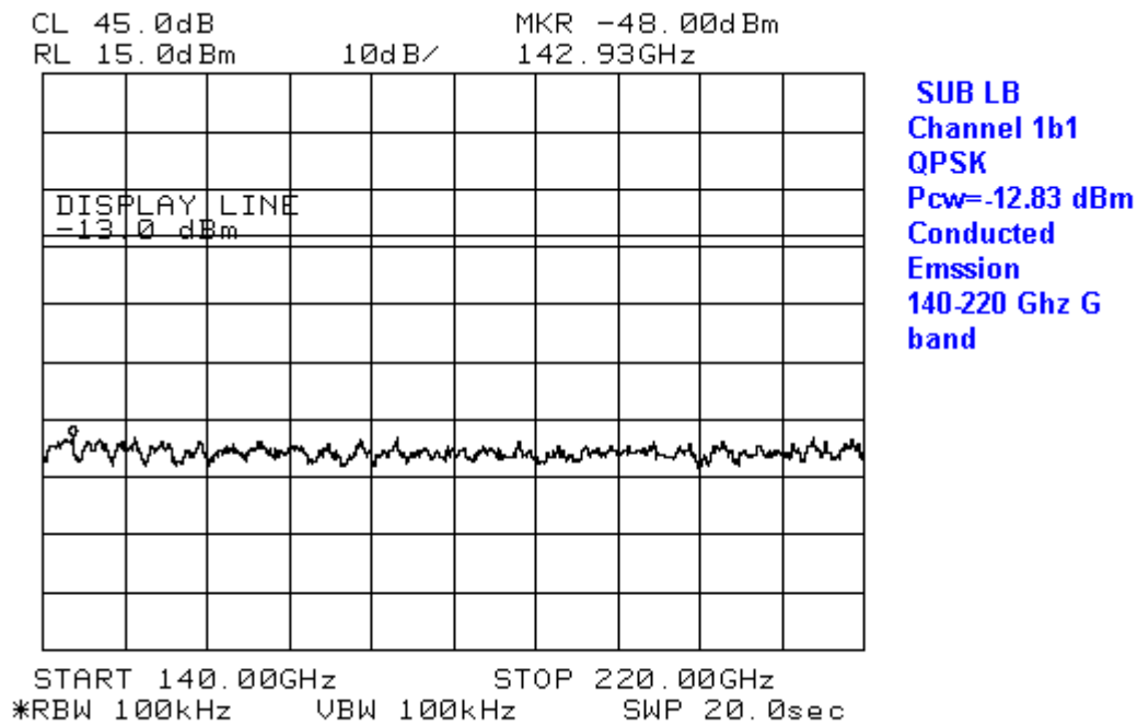
Figure 39 Conducted Emissions in 140 – 220 GHz, for transmitting -12 dBm on channel 1B1
