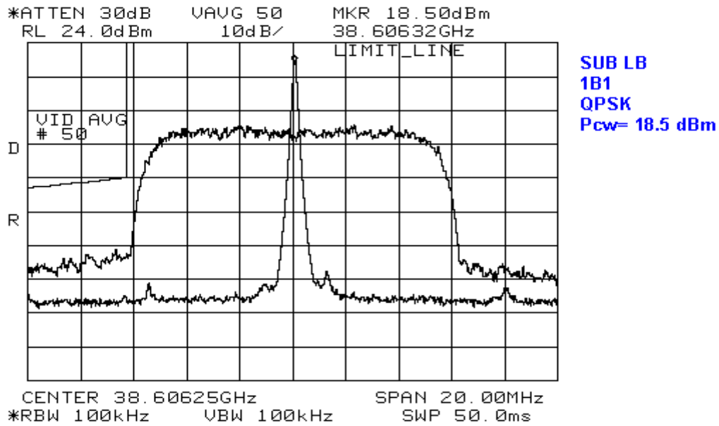
Figure 6 Output Power for QPSK modulation on ch. 1B1
