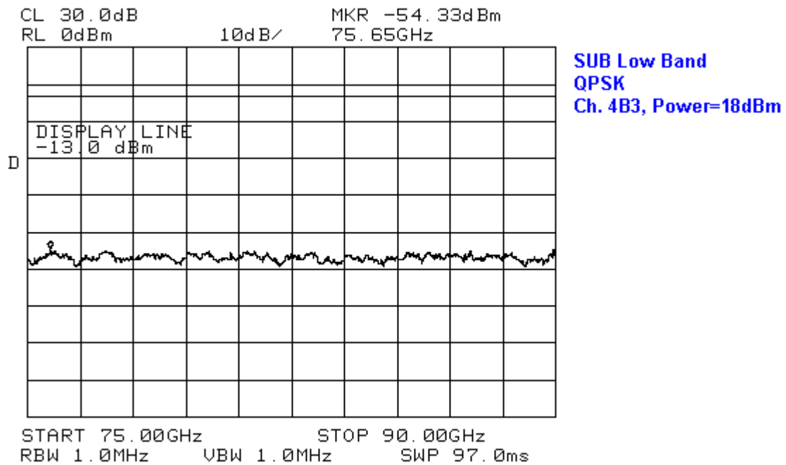
Figure 51 Radiated Emissions in 75 – 90 GHz, for transmitting 18 dBm on channel 4B3
