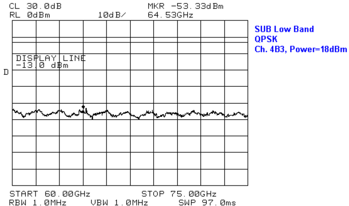
Figure 59 Radiated Emissions in 60 – 75 GHz, for transmitting 18 dBm on channel 4B3
