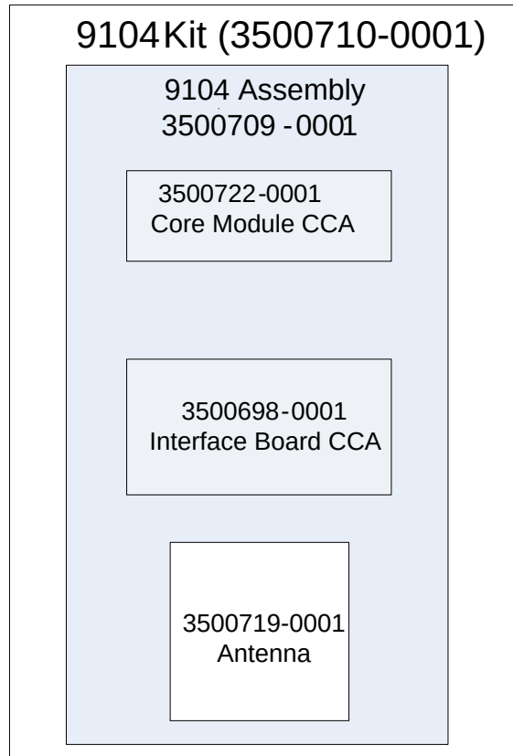
Figure 2-1: 9104 Kit breakdown
