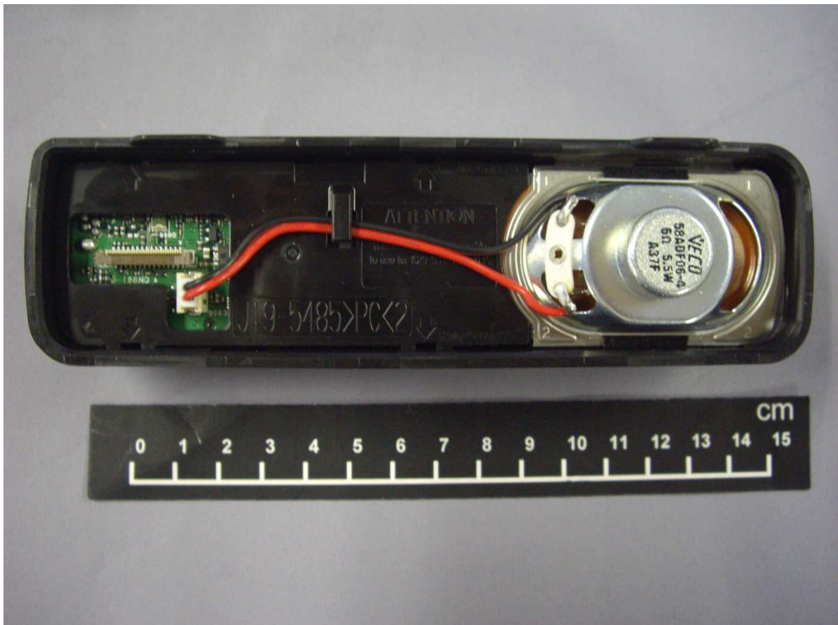
Front Internal View of Display Unit
