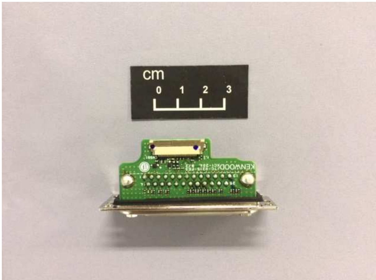
Upper side of D-Sub Unit
