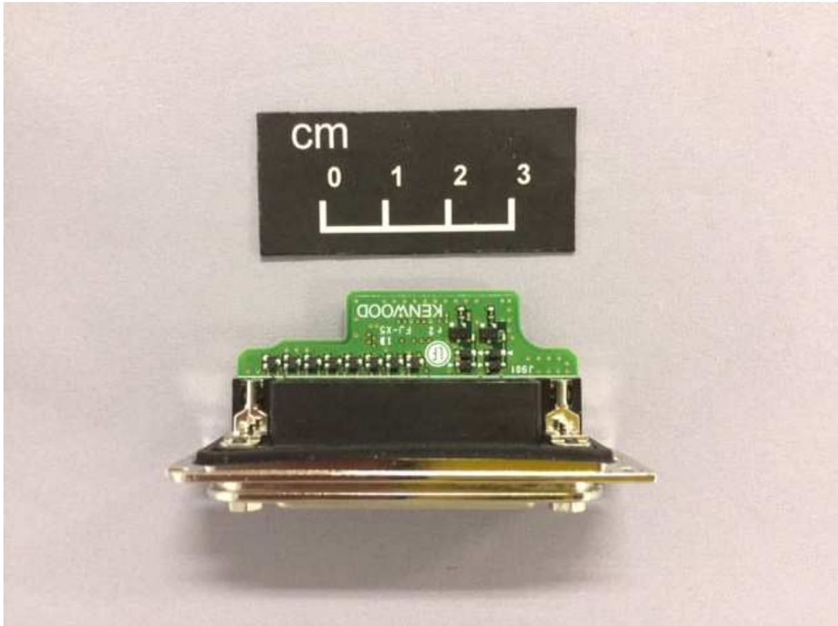
Bottom side of D-Sub Unit
