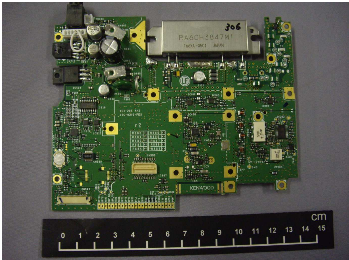
Upper side of Main Unit
