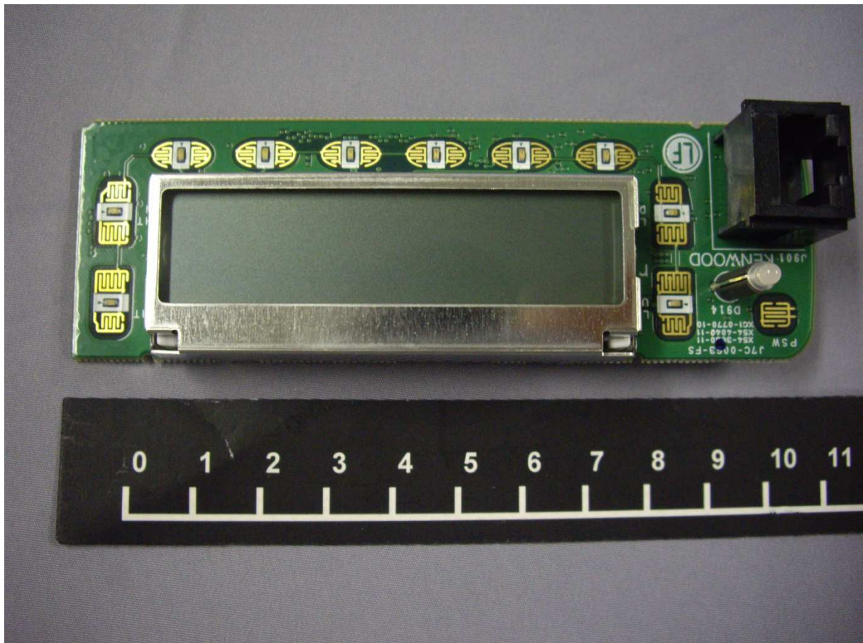
Bottom side of Display Unit
