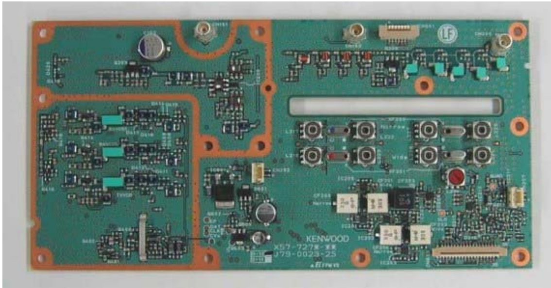
TXRX Unit Component Side View
