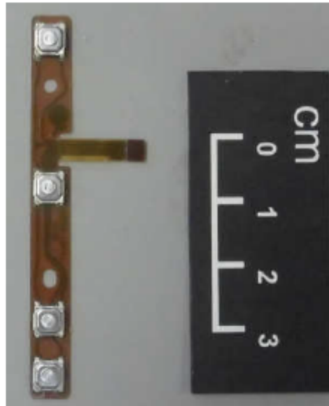
NX-5300-K2, K3, F2, F3 Side Key
