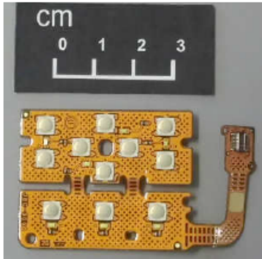
NX-5300-K2, F2 Front Key
