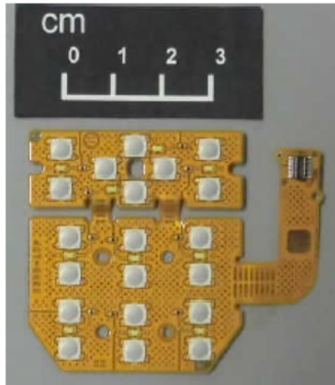
NX-5300-K3, F3 Front Key
