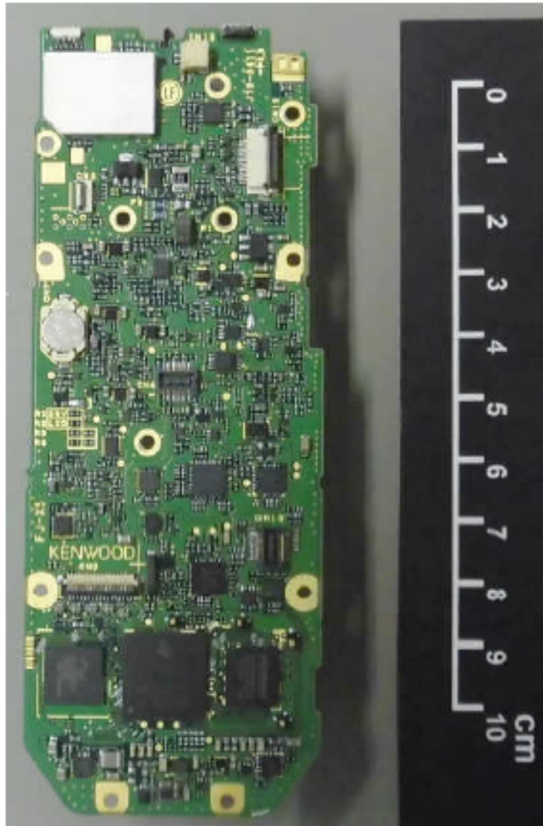
NX-5300-K2, K3, F2, F3 MAIN UNIT
