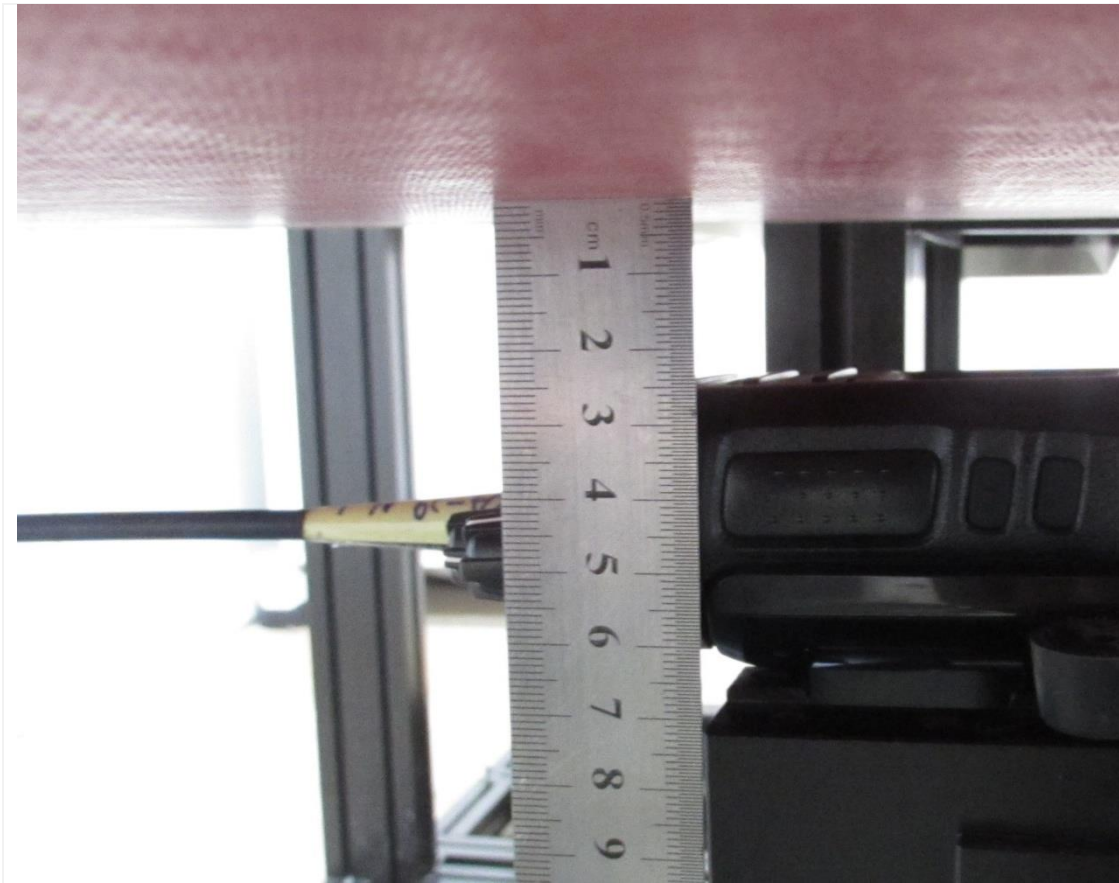
Distance of 25 mm from the EUT
