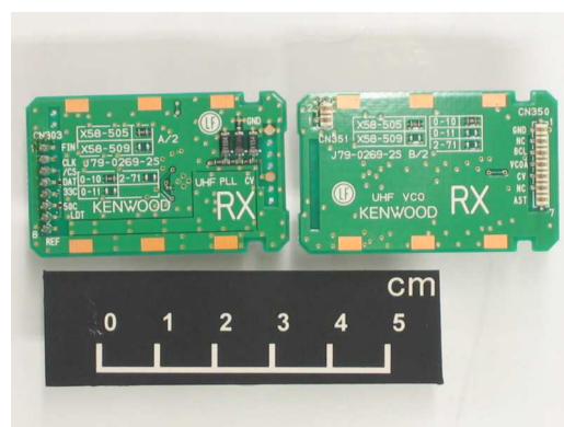
SUB RX VCO/PLL Foil Side View
