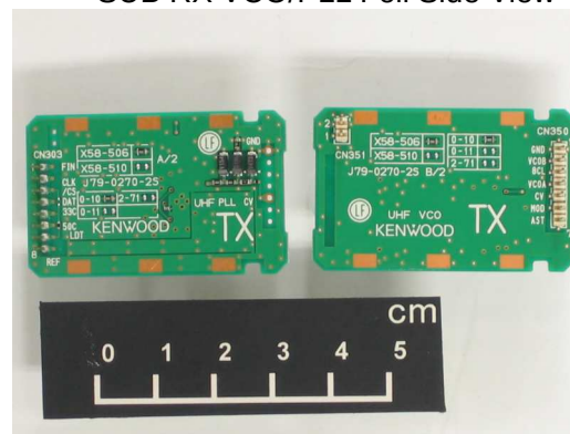
SUB TX VCO/PLL Foil Side View
