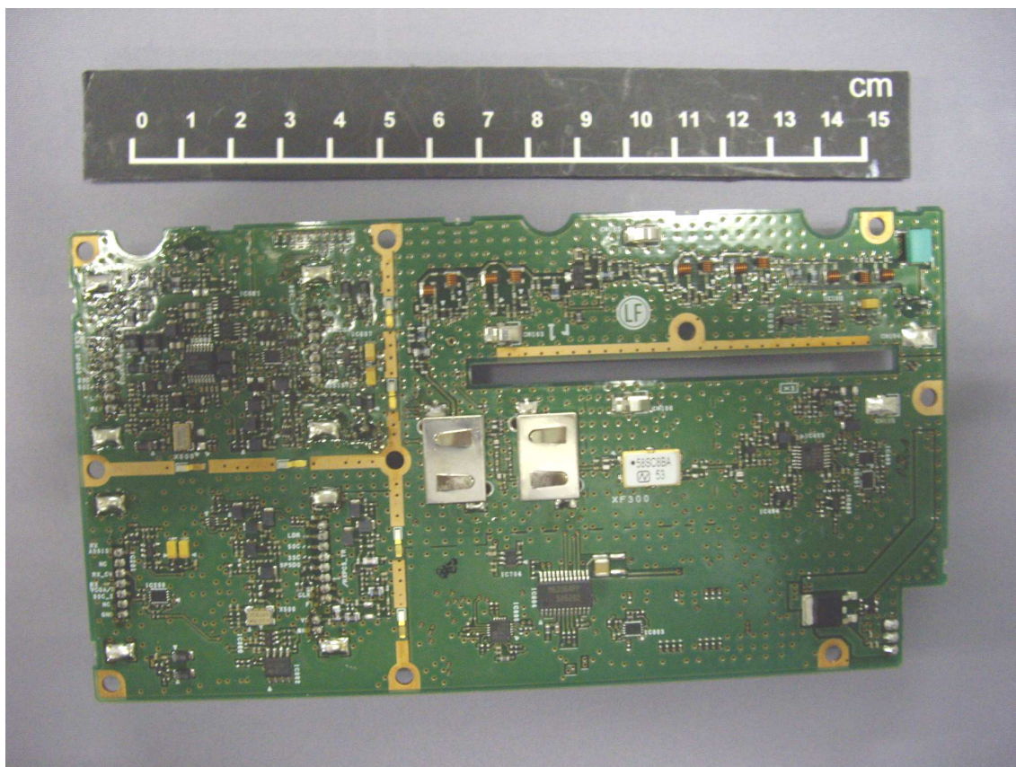
TX-RX Foil Side View
