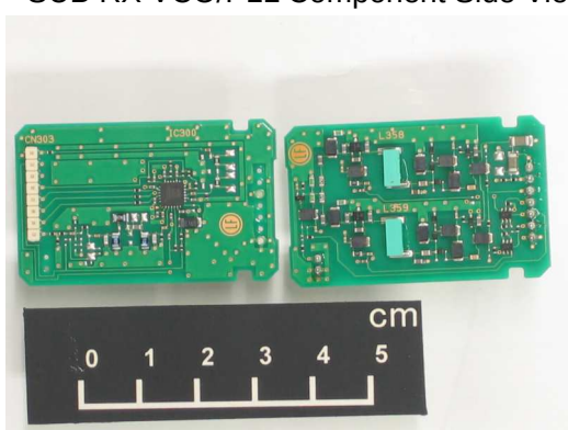
SUB TX VCO/PLL Component Side View
