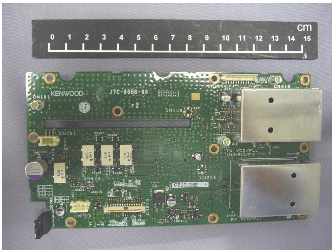
TX-RX Component Side View
