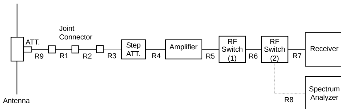
Diagram of the measurement instruments ( 1000 - 1800 MHz)
