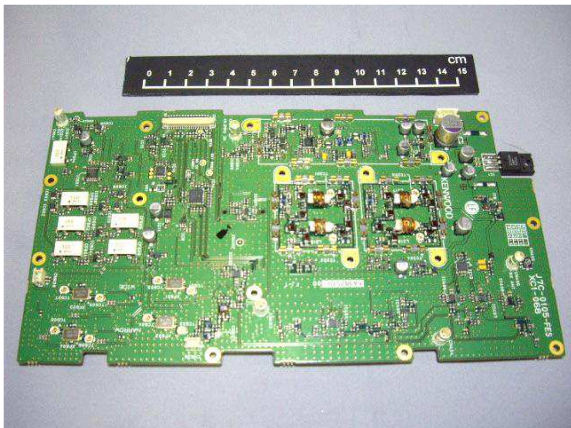
RX Upper Side View
