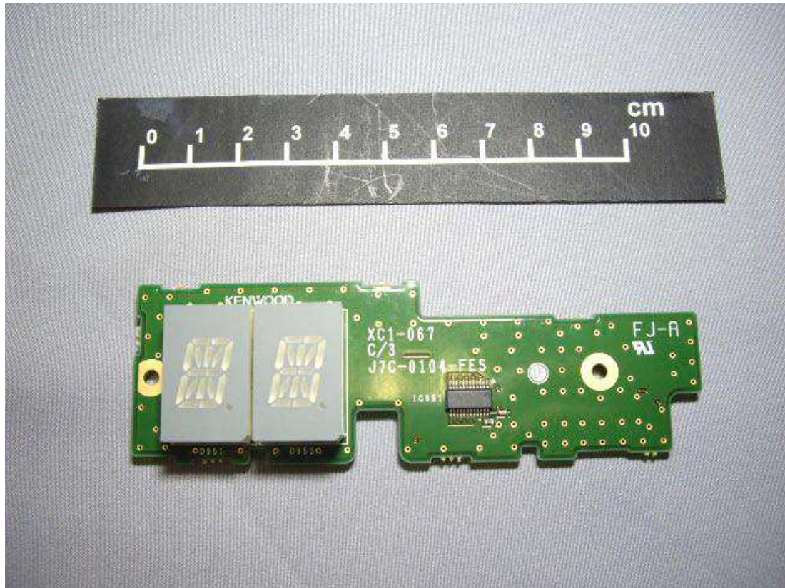
TX3 Upper Side View
