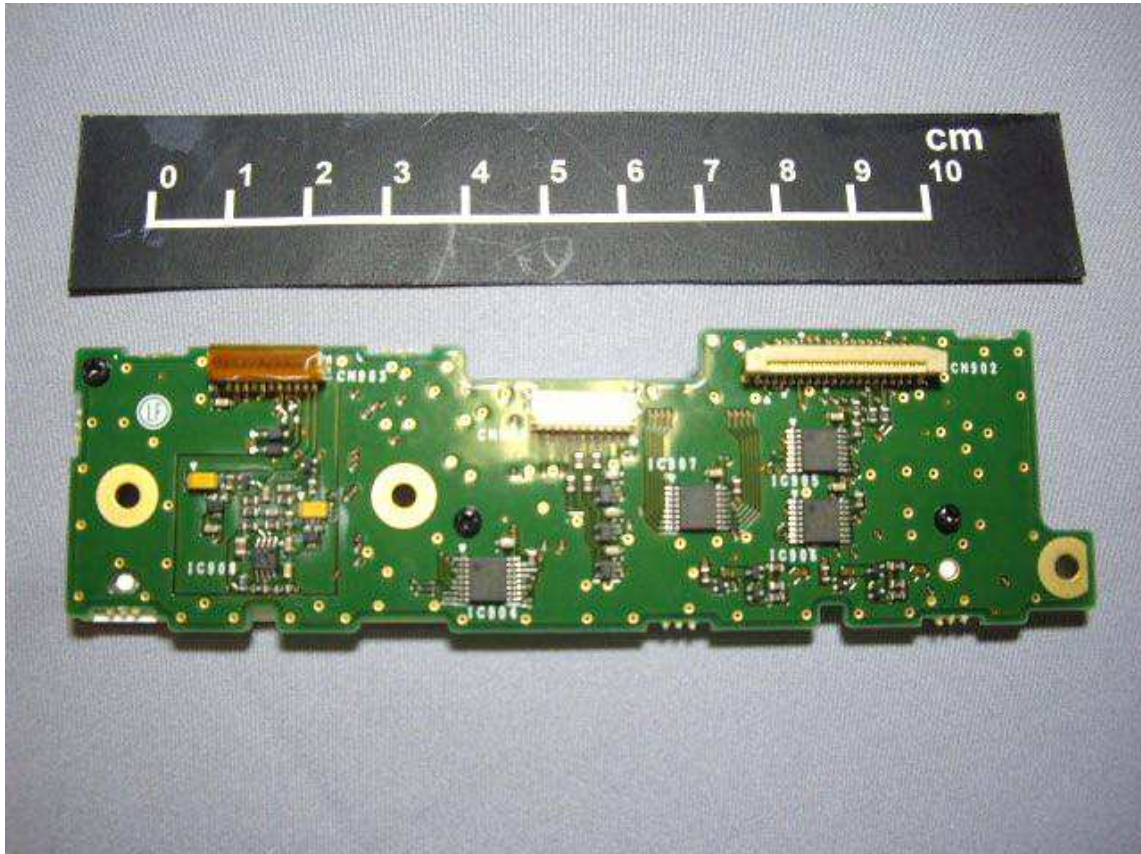
TX2 Bottom Side View
