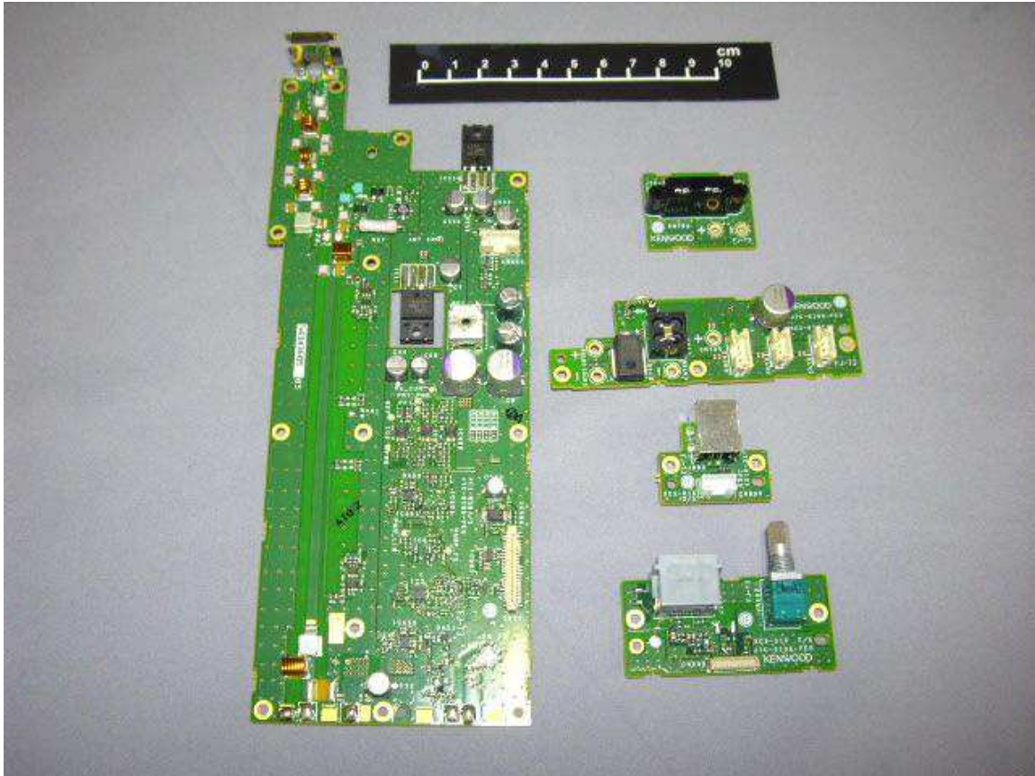
Final1-5 Upper Side View
