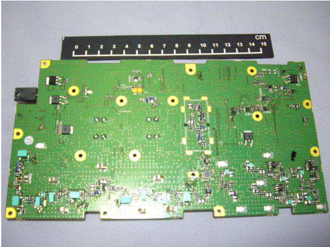
RX Bottom Side View
