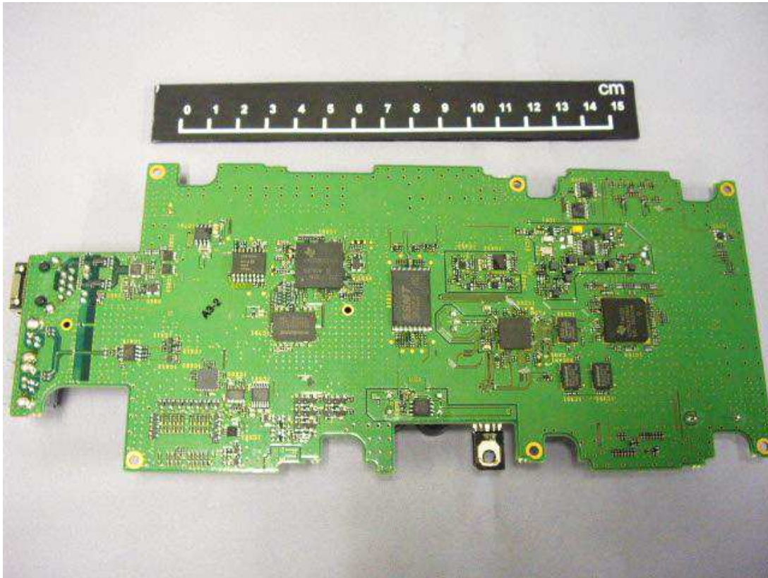
Control Bottom Side View
