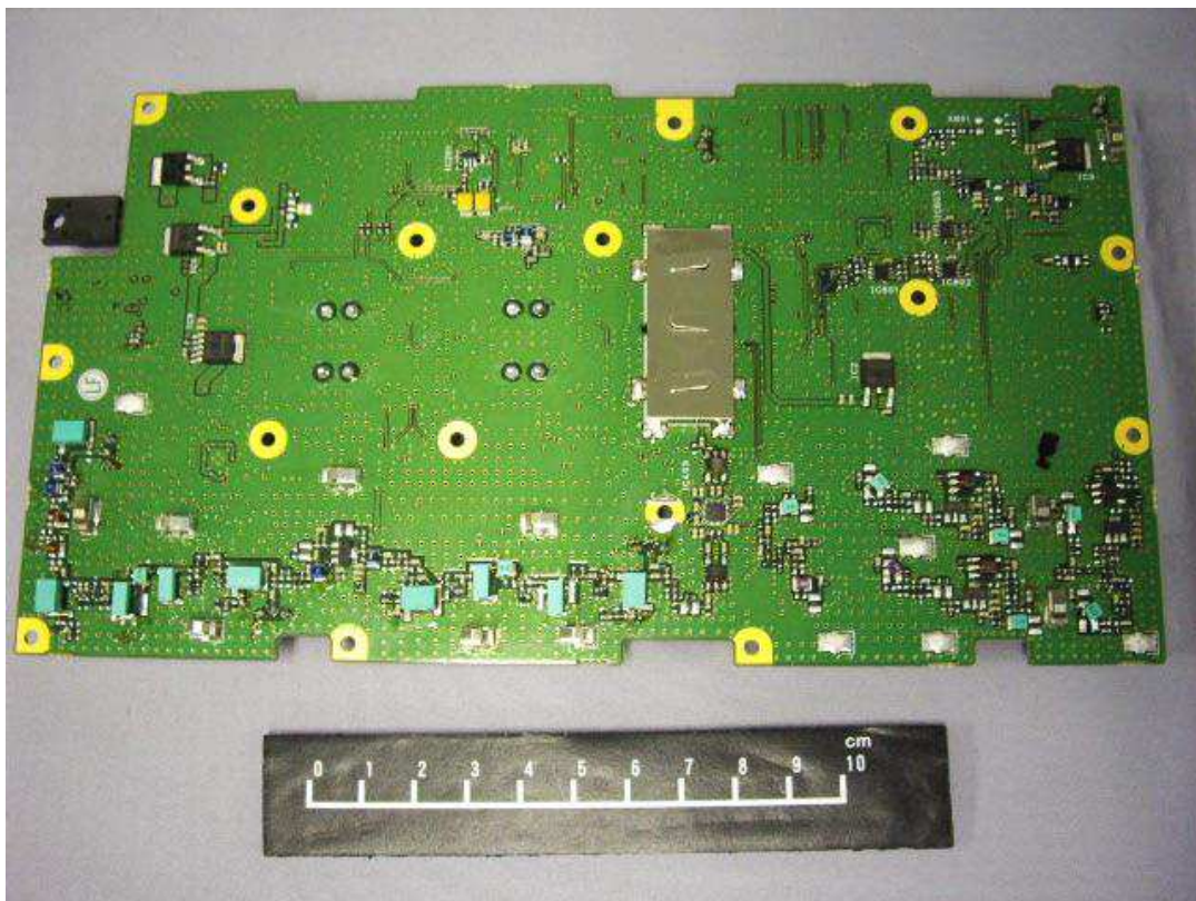
RX Bottom Side View with Shield
