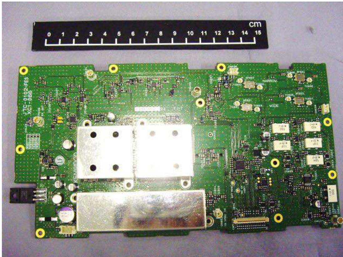
RX Upper Side View with Shield
