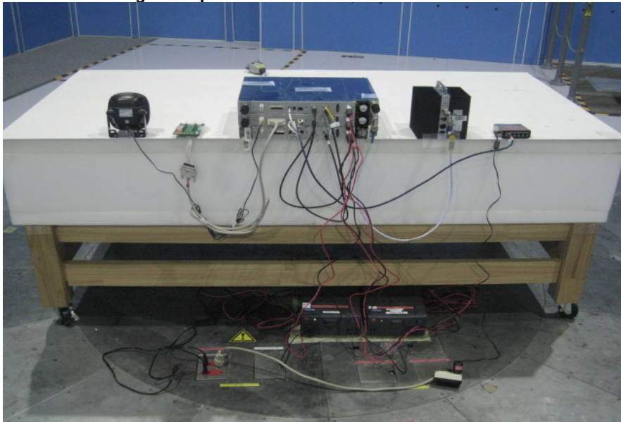
10.3 Field Strength of Spurious Radiation : Rear view
