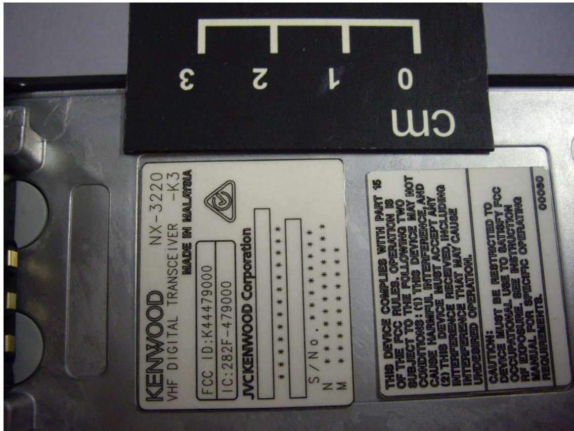
MODEL NAME PLATE and CAUTION STICKER of NX-3220-K3
