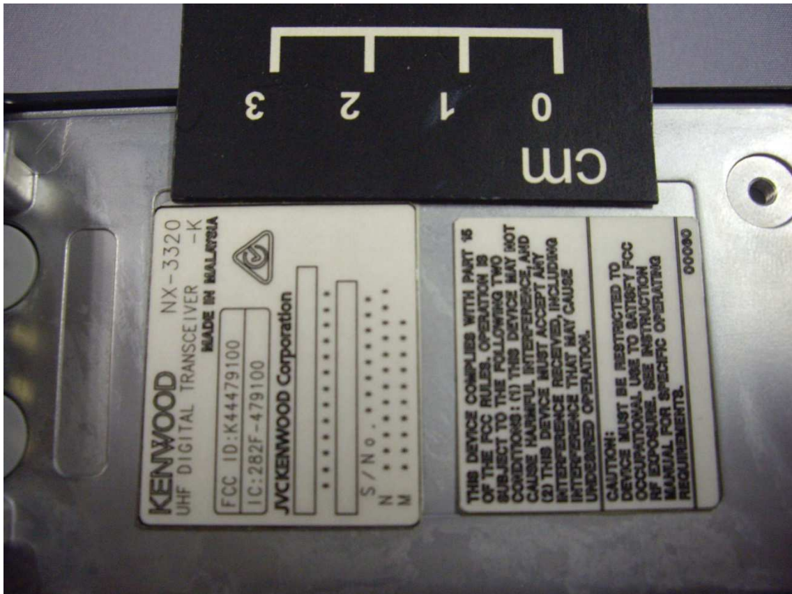
MODEL NAME PLATE and CAUTION STICKER of NX-3320-K
