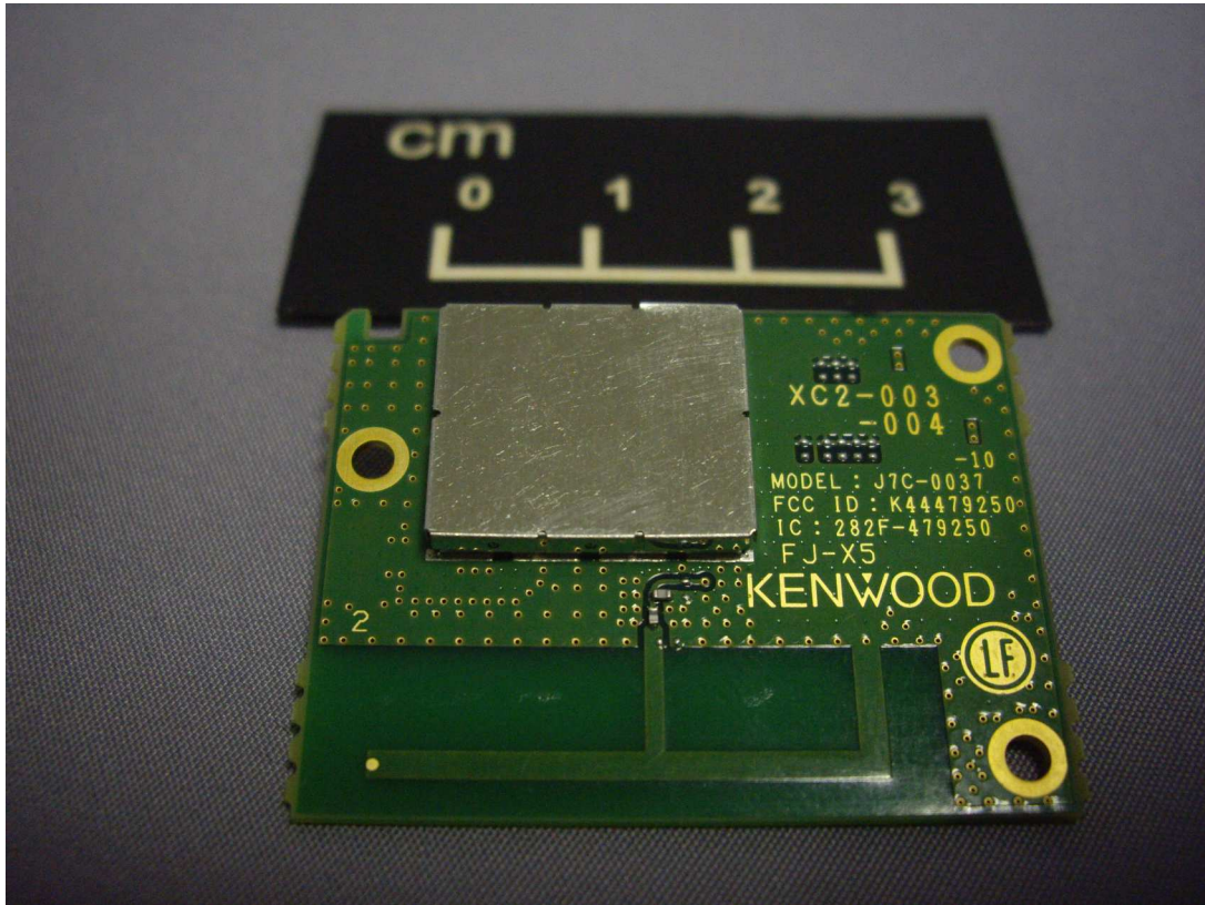
Bluetooth Module (Top)
