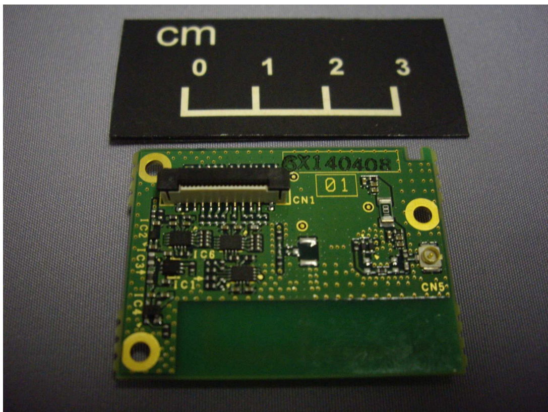
Bluetooth Module (Bottom)
