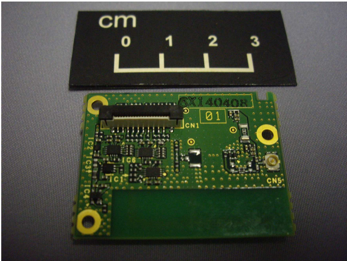
Bluetooth Module (Bottom)
