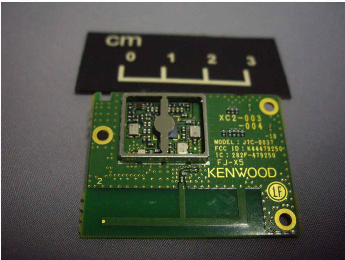
Bluetooth Module without Shield case (Top)
