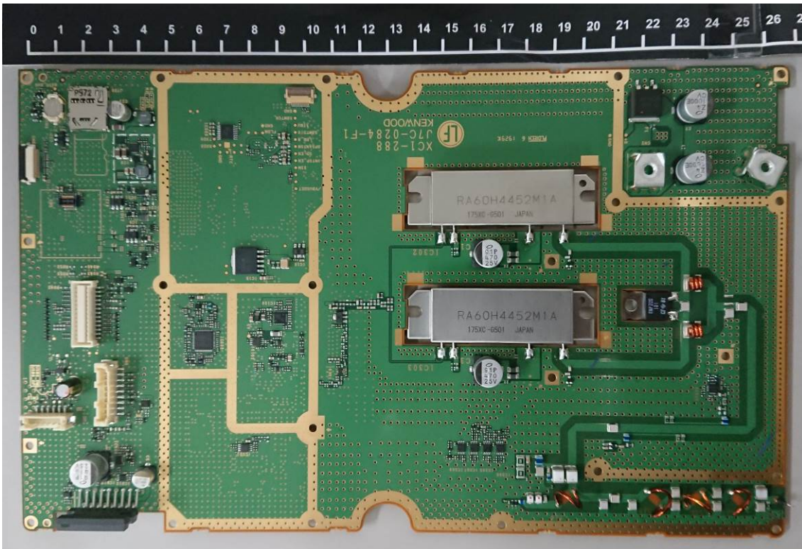
MAIN UNIT
