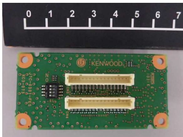
INTERFACE UNIT
