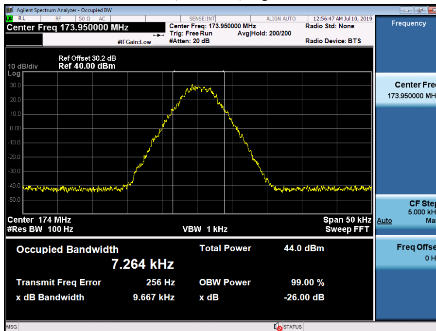
(173.95 MHz)_High
