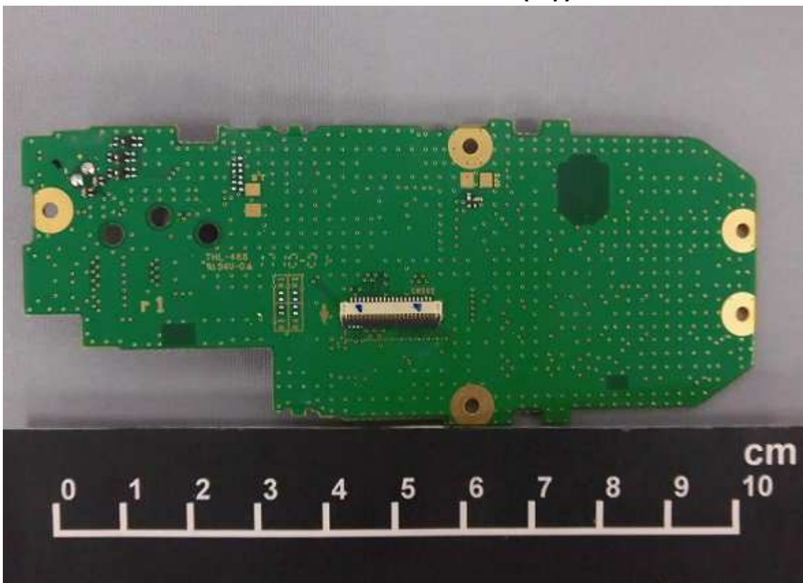
DISPLAY Unit of NX-3420-M (Bottom)
