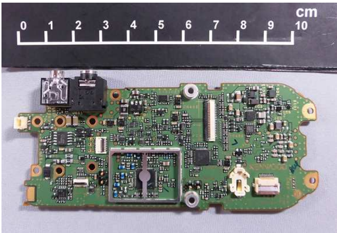
TX-RX Unit of NX-3420-M, NX-3420-M3 and NX-3420-K3 without shield case (Top)
