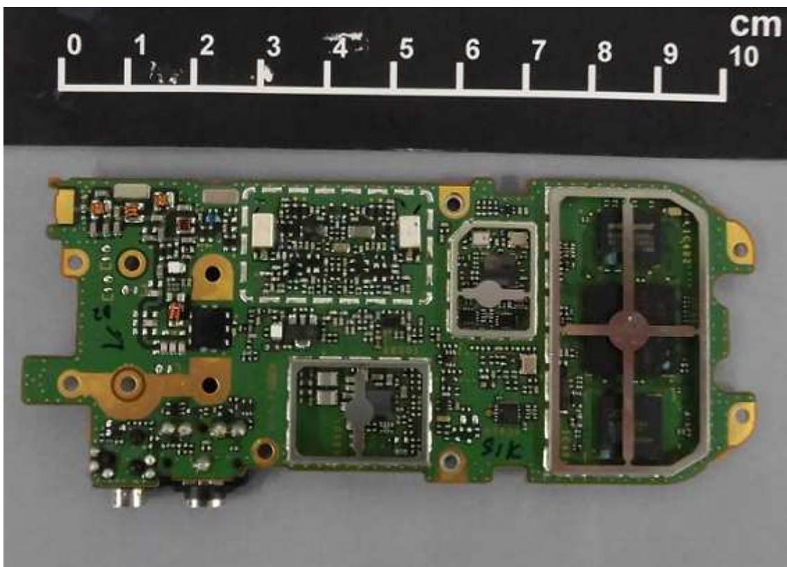
TX-RX Unit of NX-3420-M, NX-3420-M3 and NX-3420-K3 without shield case (Bottom)
