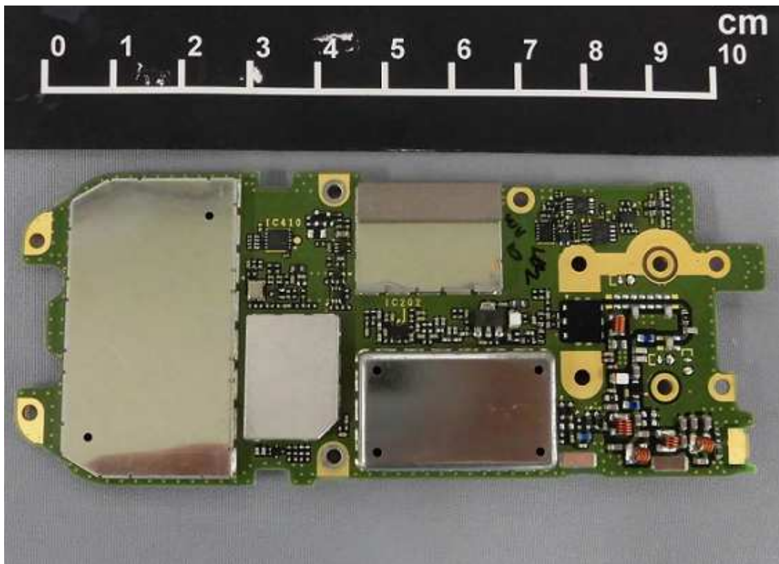
TX-RX Unit of NX-3400-K3 (Bottom)
