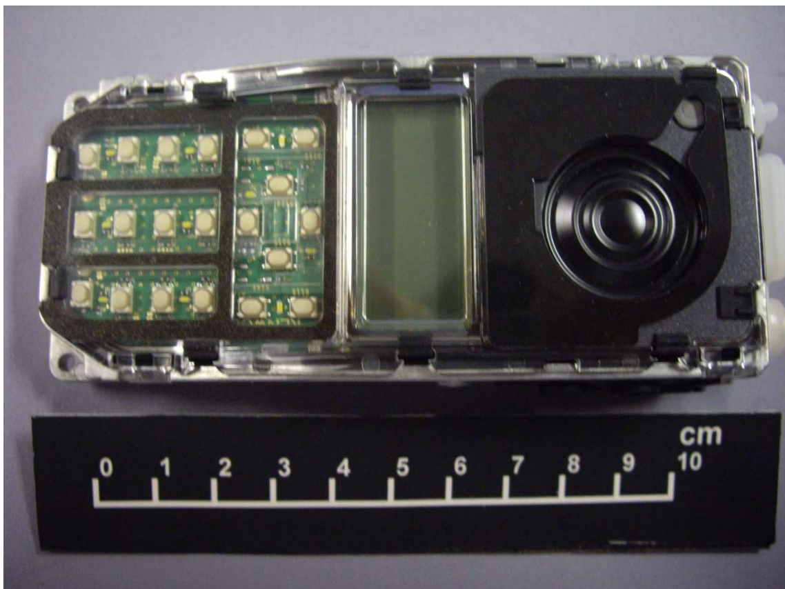
Top Internal View of NX-3400-K3, NX-3420-K3 and NX-3420-M3
