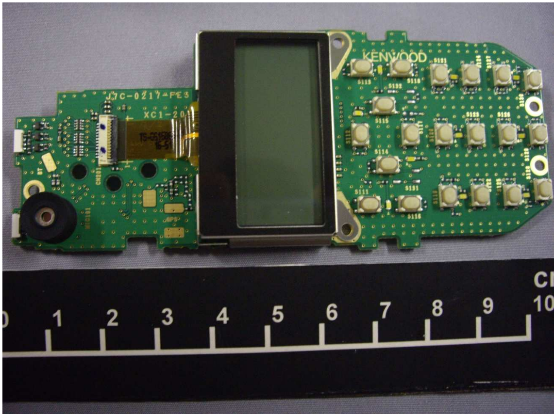
DISPLAY Unit of NX-3400-K3, NX-3420-K3 and NX-3420-M3 (Top)
