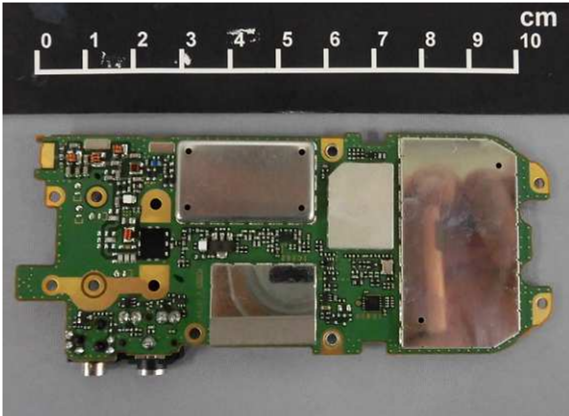
TX-RX Unit of NX-3420-M, NX-3420-M3 and NX-3420-K3 (Bottom)
