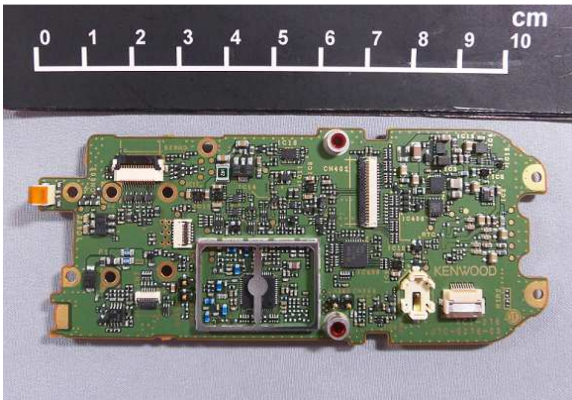
TX-RX Unit of NX-3400-K3 without shield case (Top)
