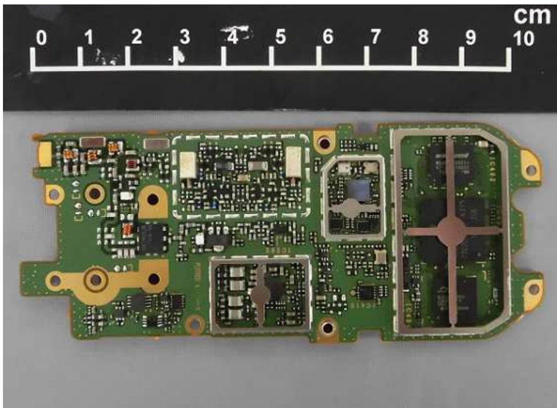
TX-RX Unit of NX-3400-K3 without shield case (Bottom)
