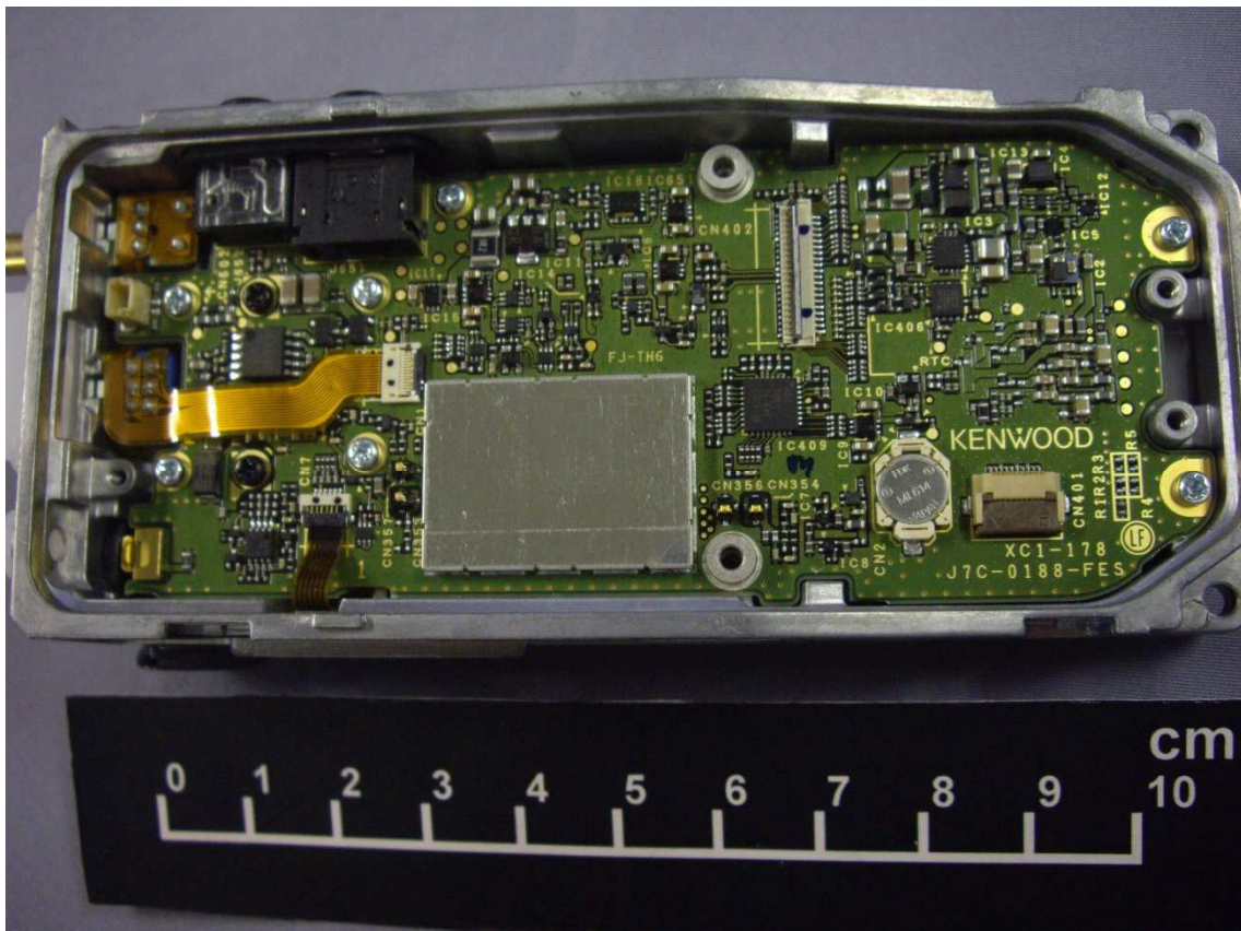
Top Internal View of TX-RX Unit (NX-3420-M, NX-3420-M3 and NX-3420-K3)
