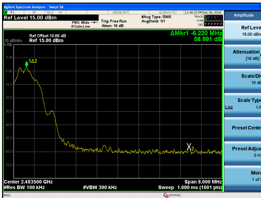
BandEdge (High-CH 39)
