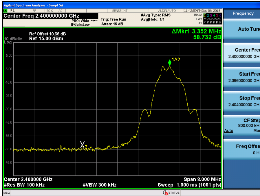
BandEdge (Low-CH 0)
