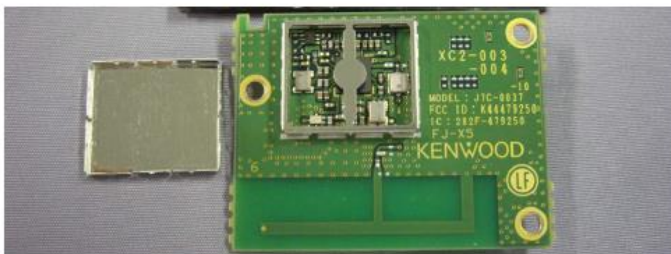
Upper side of Certified Bluetooth Module (without shield case)
