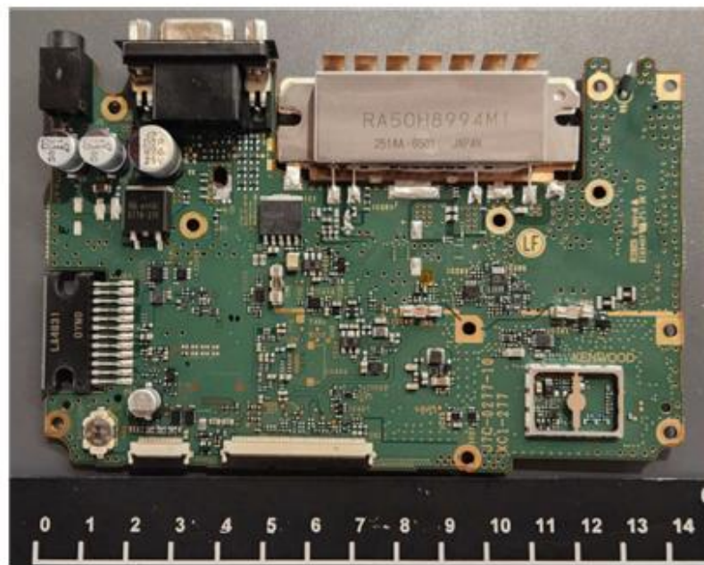
Upper side of TX-RX Unit (without shield case)
