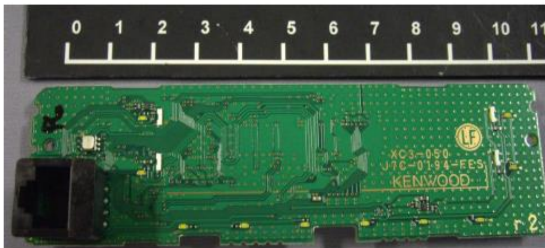
Bottom side of SUB Unit
