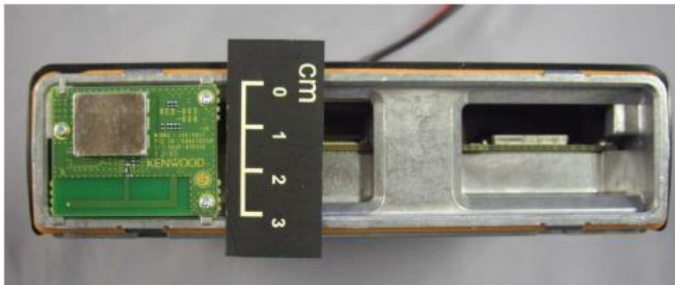
Front Internal View of Certified Bluetooth Module
