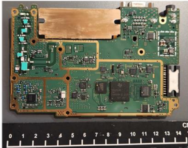
Bottom side of TX-RX Unit
