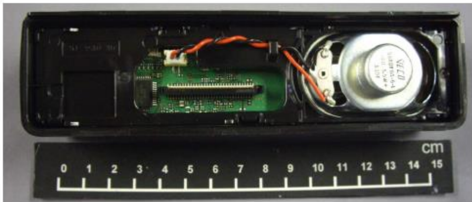
Front Internal View of SUB Unit
