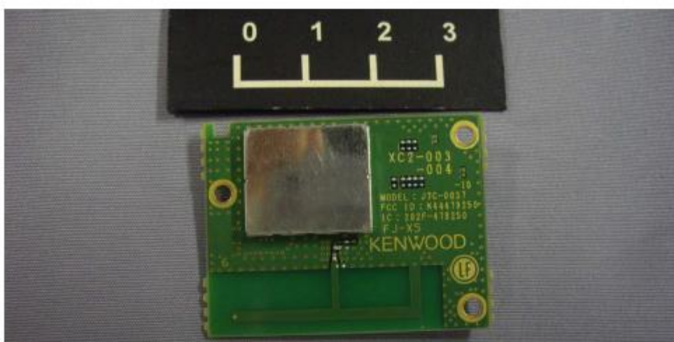
Upper side of Certified Bluetooth Module (FCC ID: K44479250, IC: 282F-479250, MODEL: J7C-0037)
