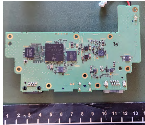
CONTROL Unit, side B
