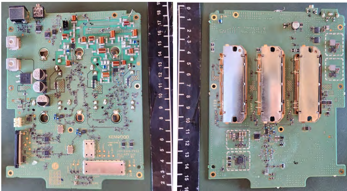
TX/RX Unit with shield case, side A
