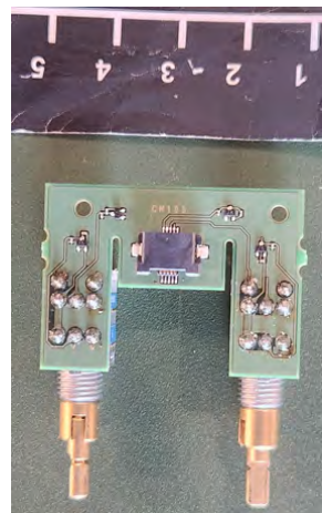
VOLUME Unit, side B
