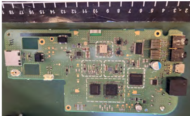
DISPLAY Unit without shield case, side A -
