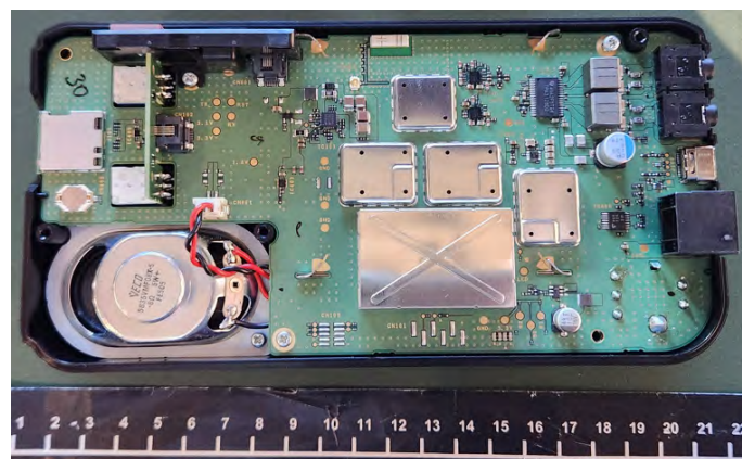
Top Internal View of DISPLAY Unit
