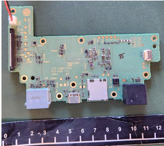
CONTROL Unit, side A
