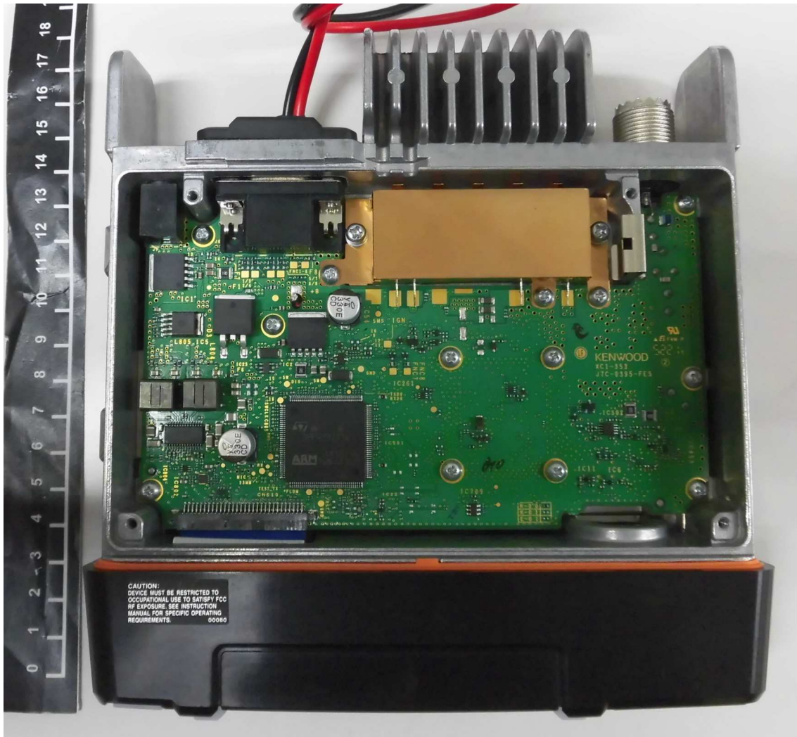
Top Internal View of MAIN Unit
