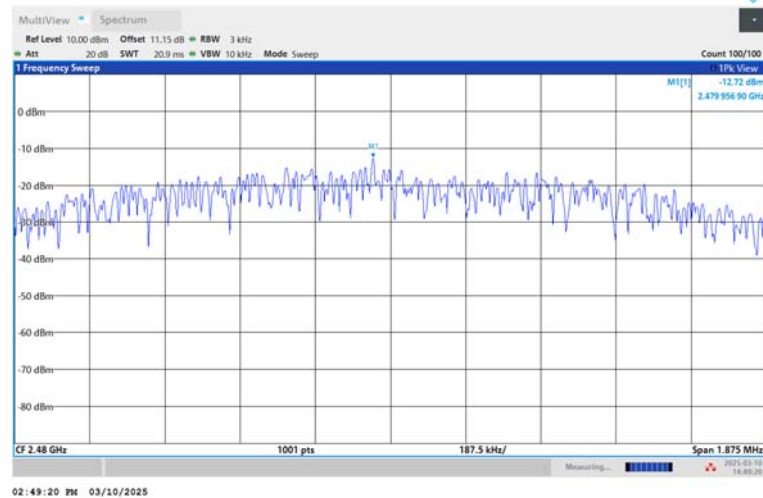
BLE_2M-Ant1-2480-PASS
