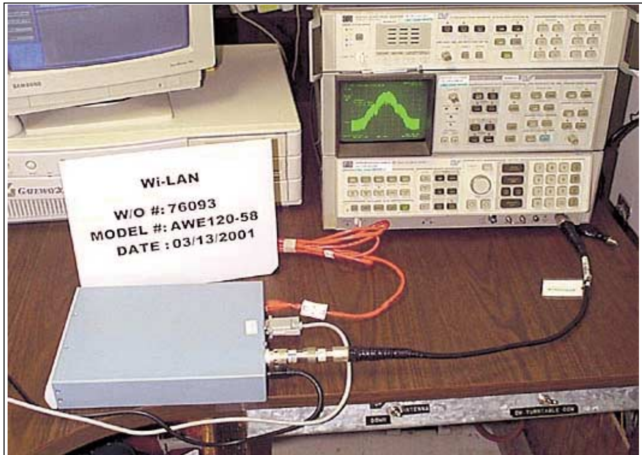
Antenna Conducted - 5MHz - 1GHz and Fundamental
