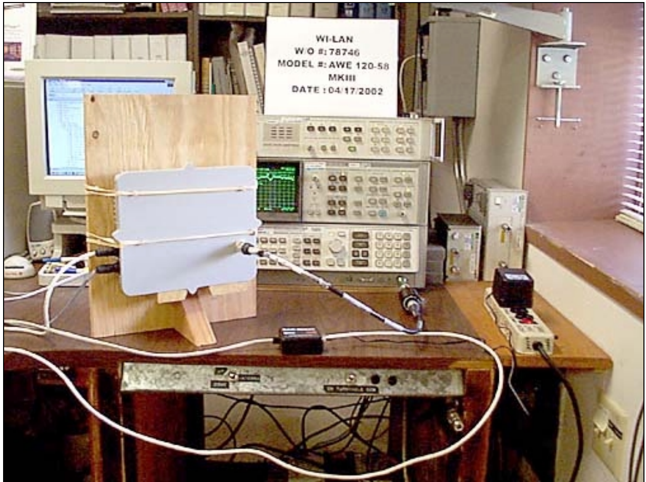
Antenna Conducted Power
