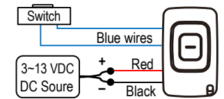
Fig. 3 External switch and built-in button
