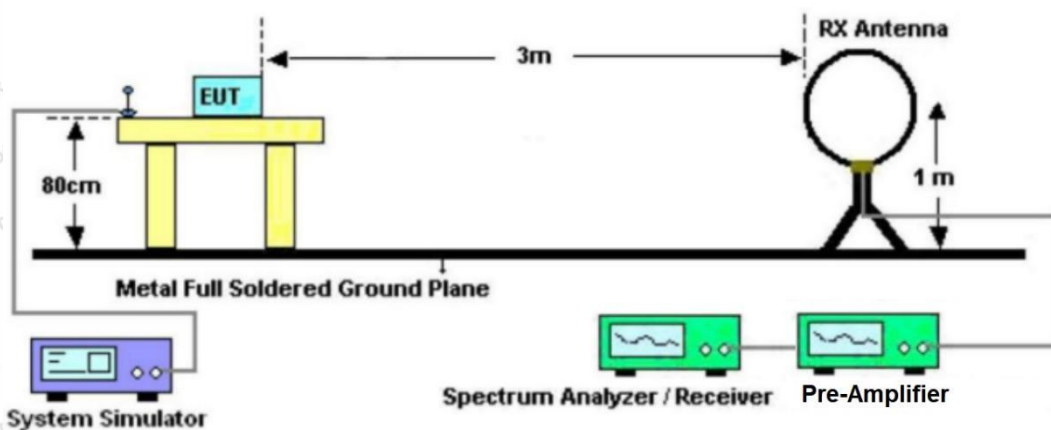
Figure 1. Below 30MHz
