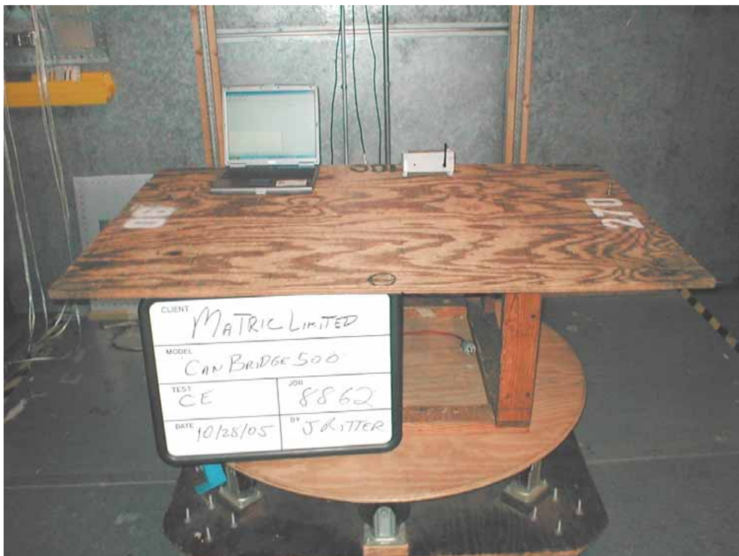
Conducted Emissions Test Setup, Photograph #1
