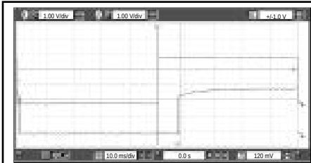
Figure 4: Power-On Timing
