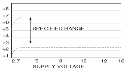
Figure 9: Output Power vs. Supply Voltage
