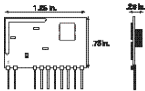
Figure 10: Physical package
