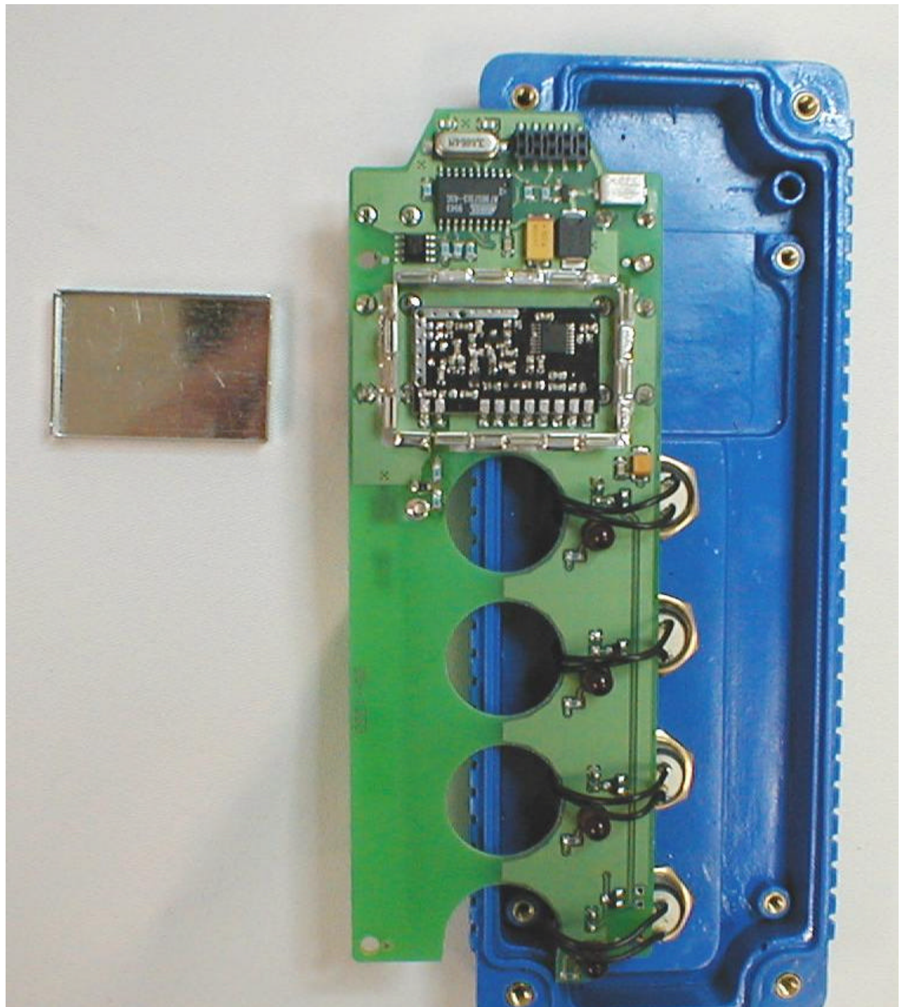
TP100 Shield Removed
