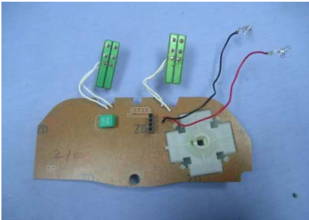
Internal of TX- 3
