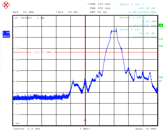
Tx 2402 MHz DH5
