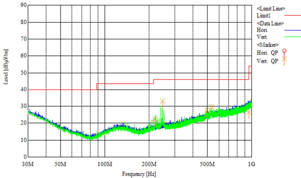
[Chart] Tx 2402MHz 2DH5 Z-plane
