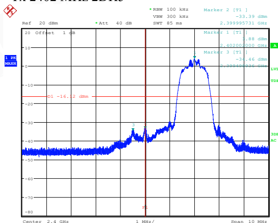
Tx 2402 MHz 2DH5
