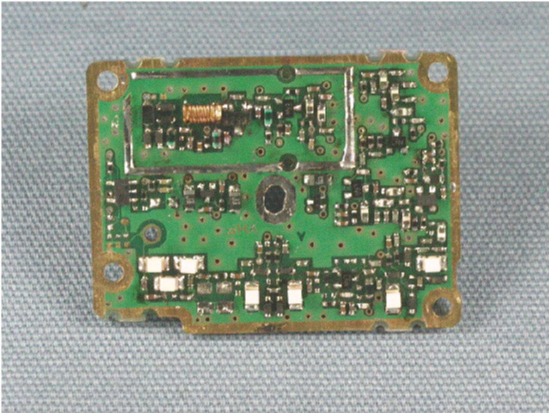
Side-B of SRX-4 (Option)
