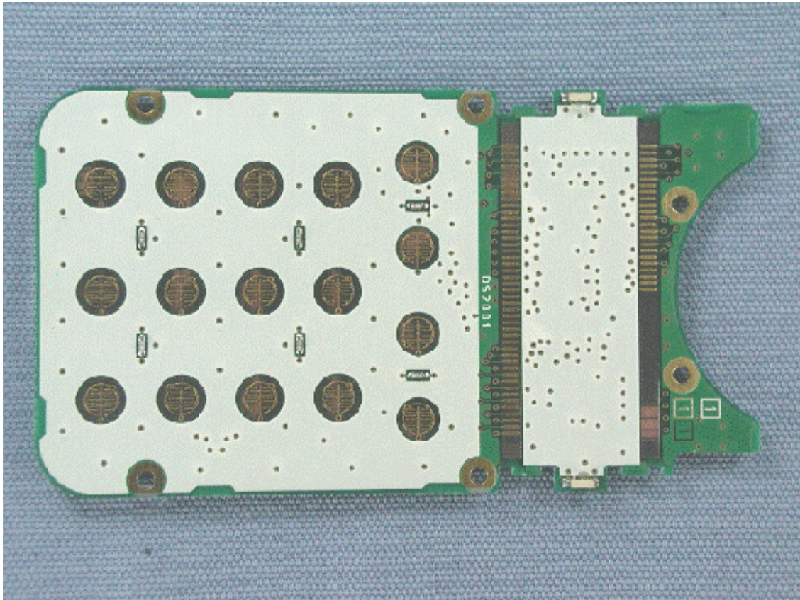
Side-A of DISPLAY-UNIT without LCD (VX-924/929/VX-974/979)
