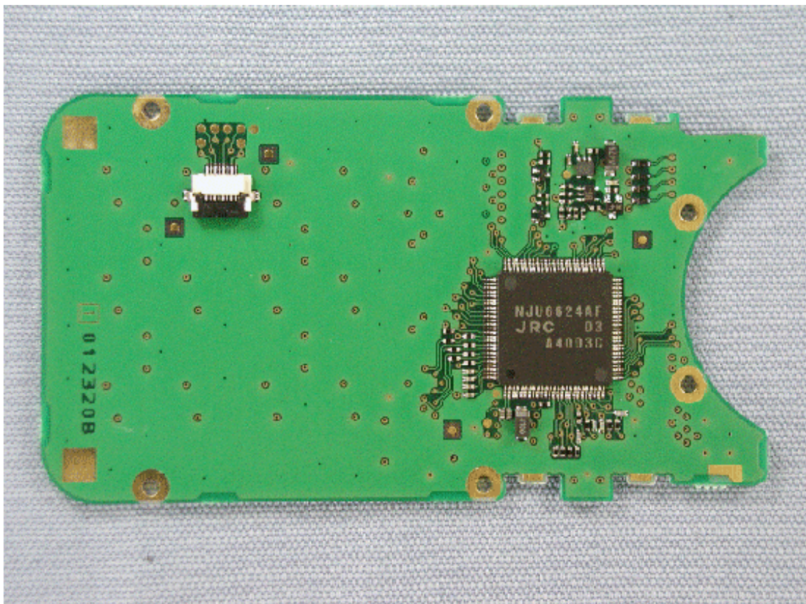
Side-B of DISPLAY-UNIT (VX-924/929/VX-974/979)
