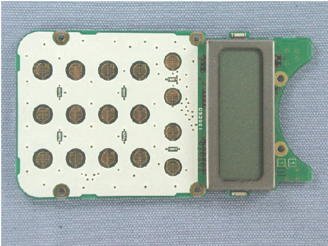
Side-A of DISPLAY-UNIT with LCD (VX-924/929/VX-974/979)
