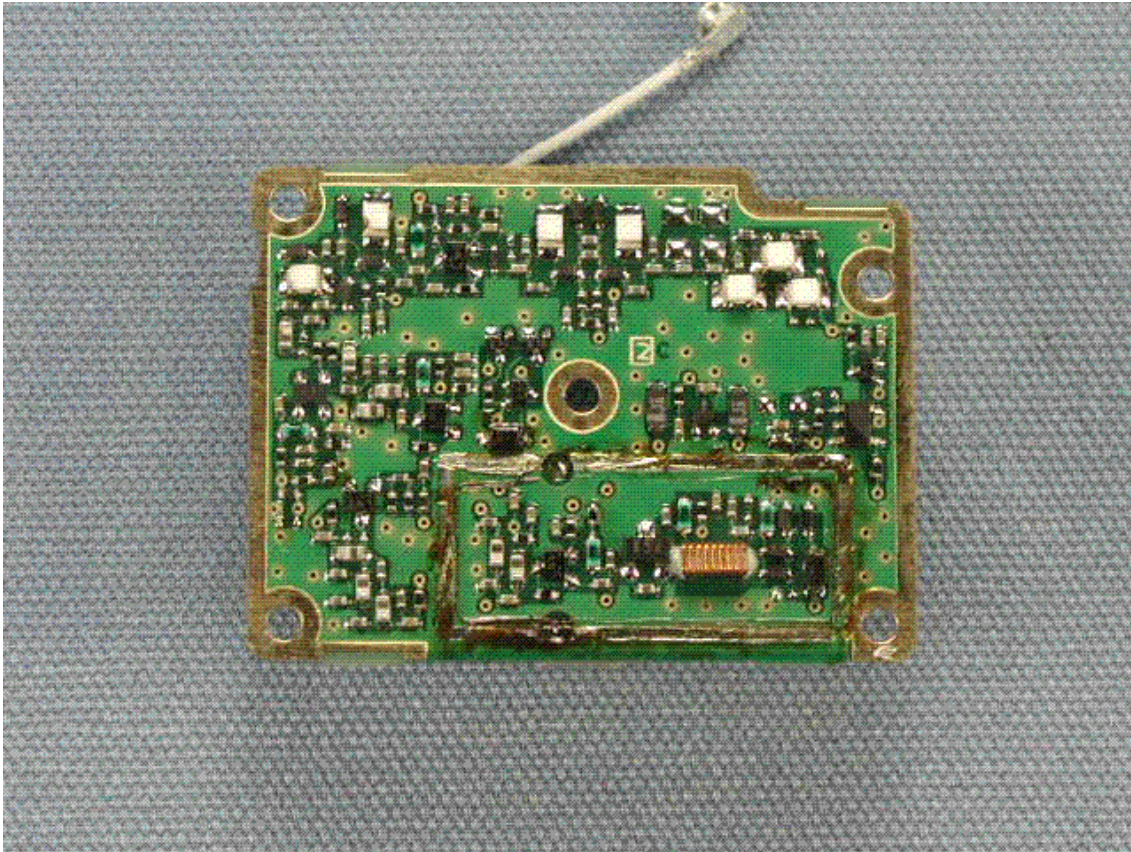
Side-B of SUB-RX-UNIT without shield case
