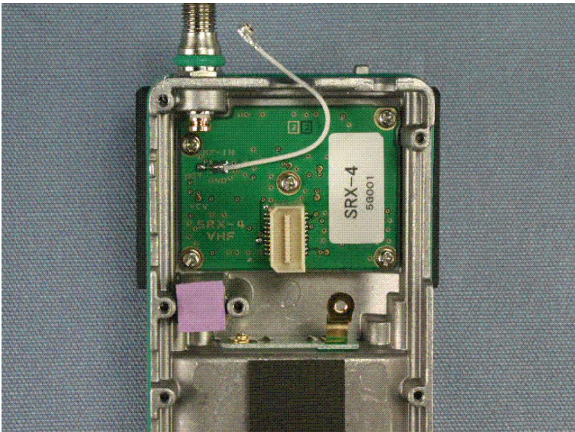
SUB-RX-UNIT in chassis
