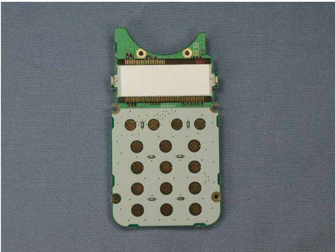
Side-A of DISPLAY-1-UNIT without LCD
