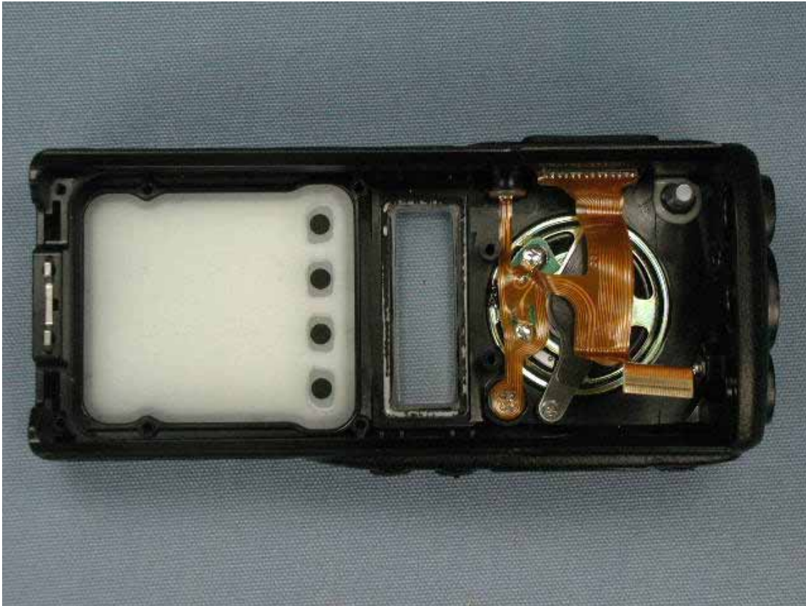
Inside of front panel (for VX-P924/P974)
