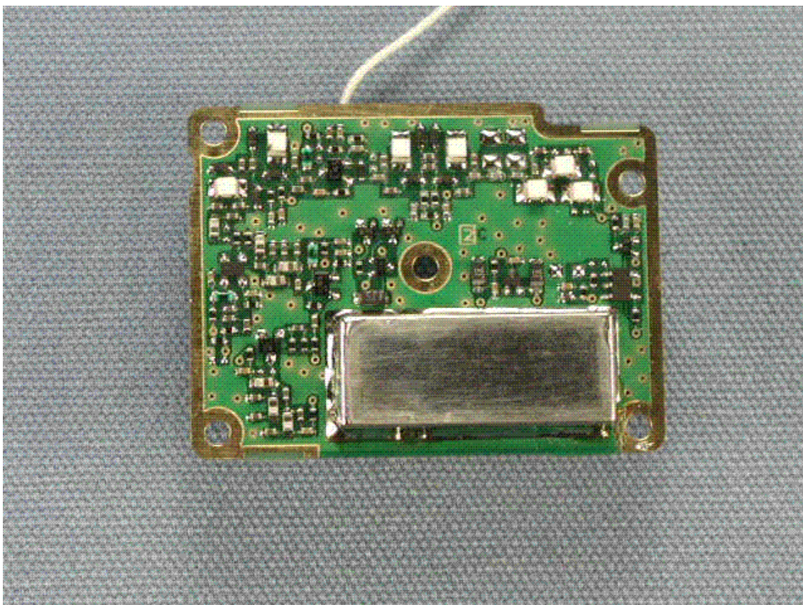
Side-B of SUB-RX-UNIT with shield case
