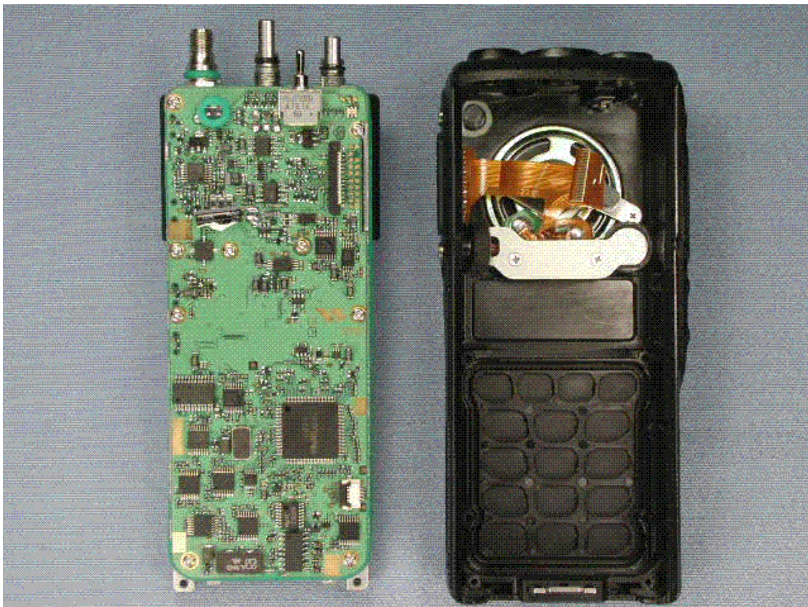
Inside view (VX-P921/P971)
