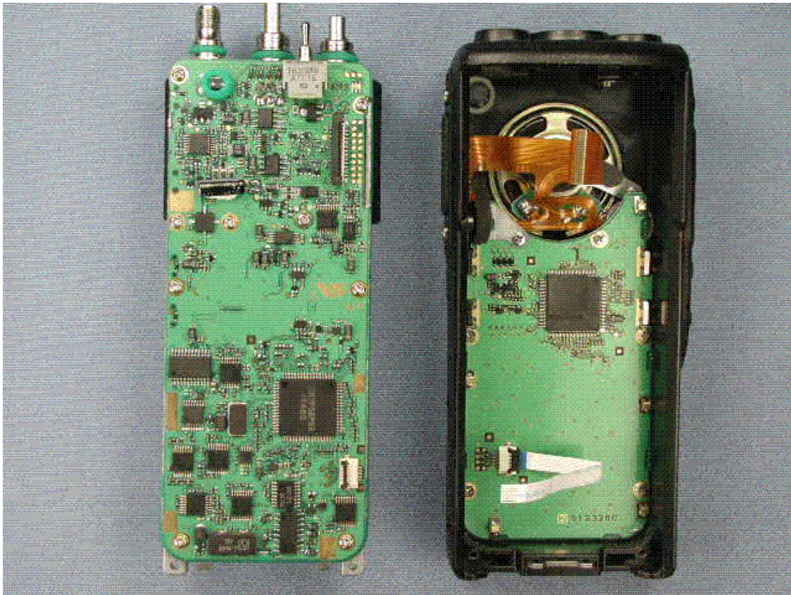
Inside view (VX-P929/P979/P924/P974)
