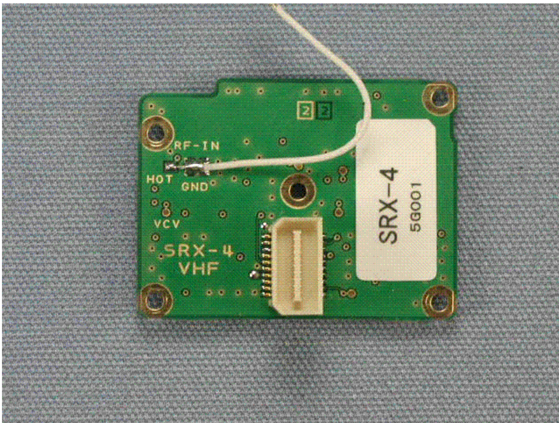
Side-A of SUB-RX-UNIT
