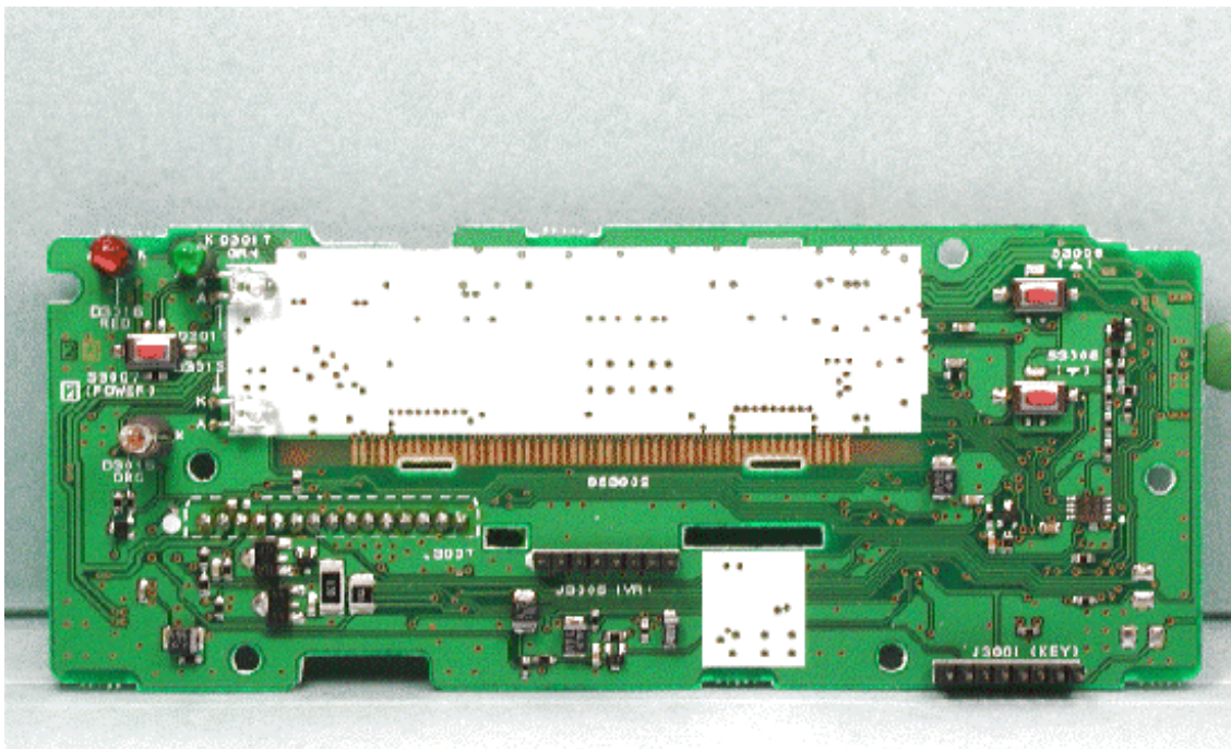
Side-A of DISPLAY-UNIT without LCD
