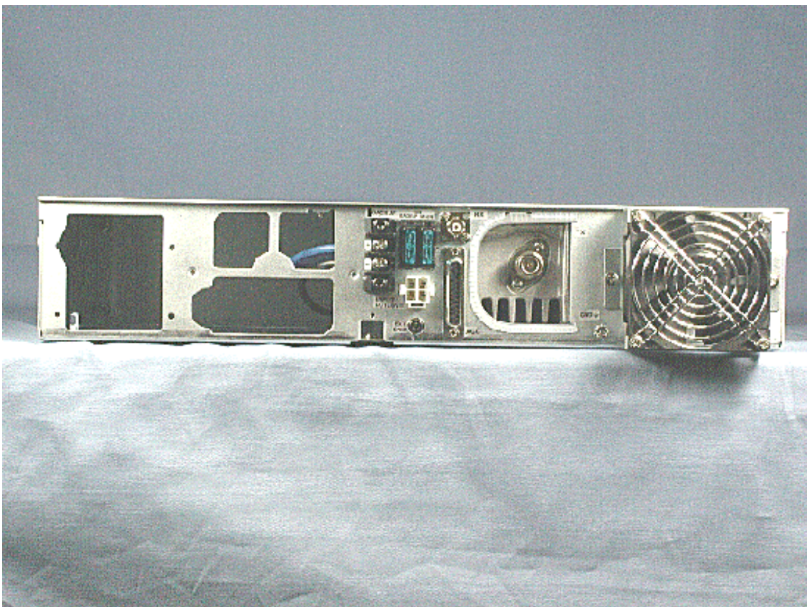
Rear view
