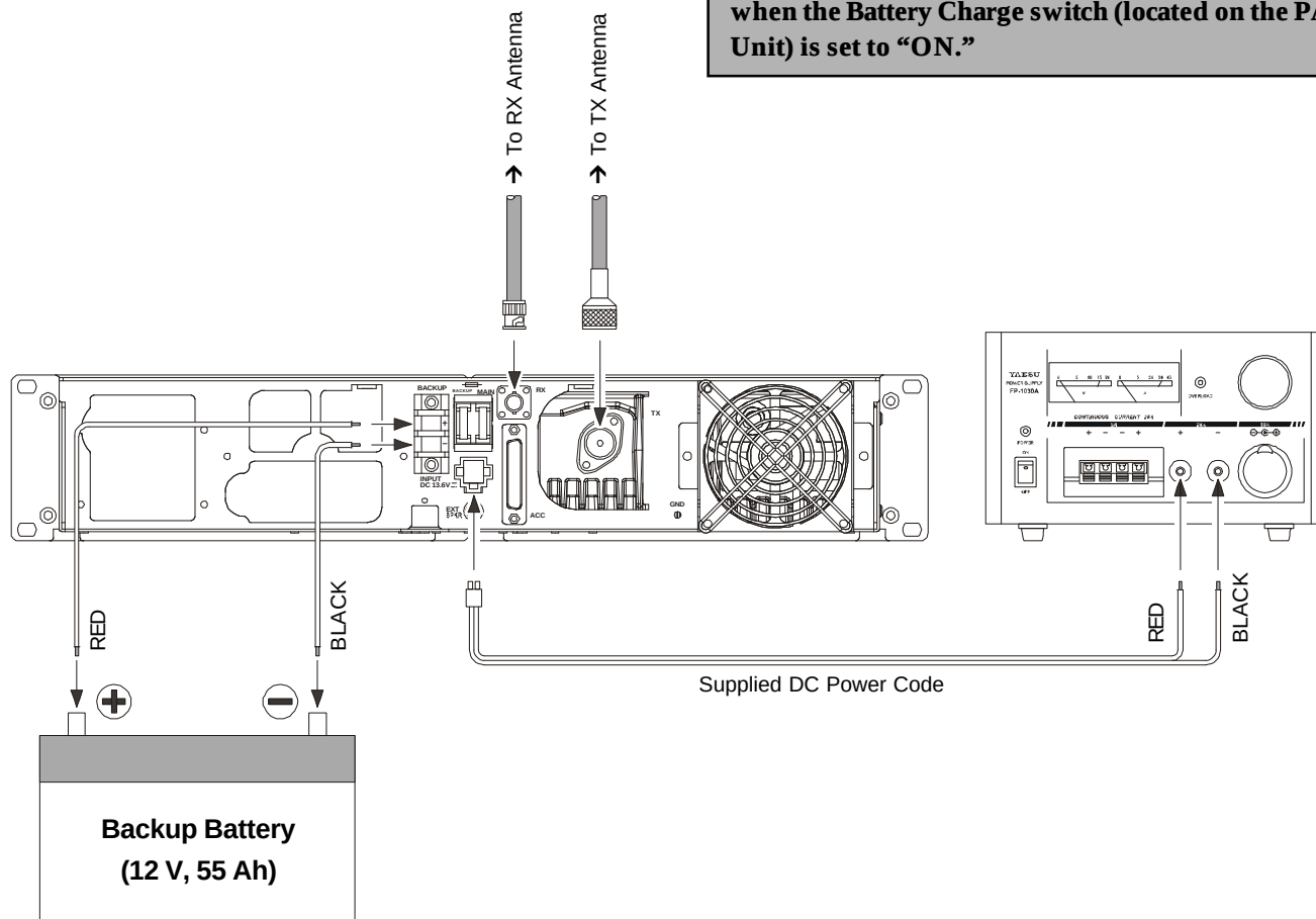
TYPICALLY SETUP
