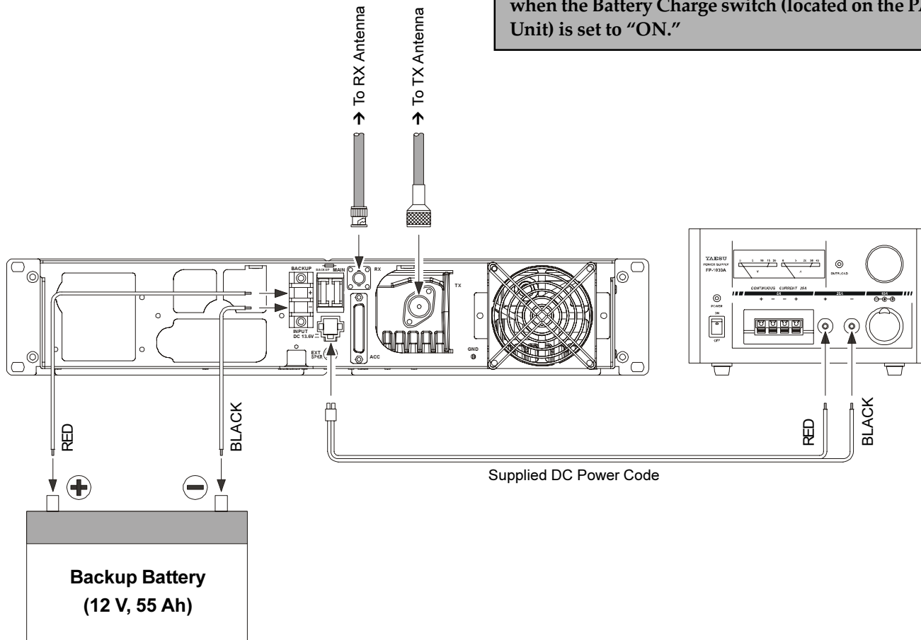
TYPICALLY SETUP
