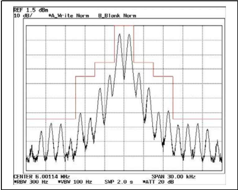
Frequency 6.0 MHz MASK A
