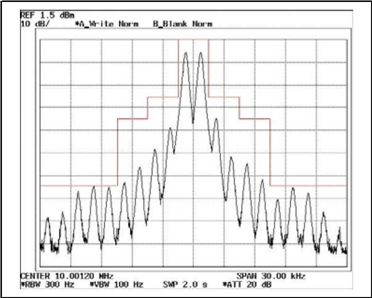
Frequency 10.0 MHz MASK A
