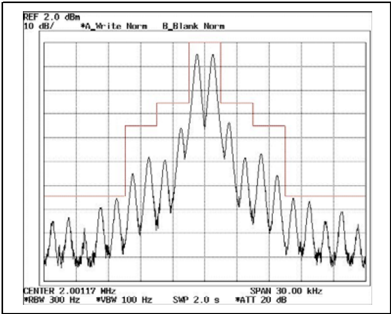
Frequency 2.0 MHz MASK A
