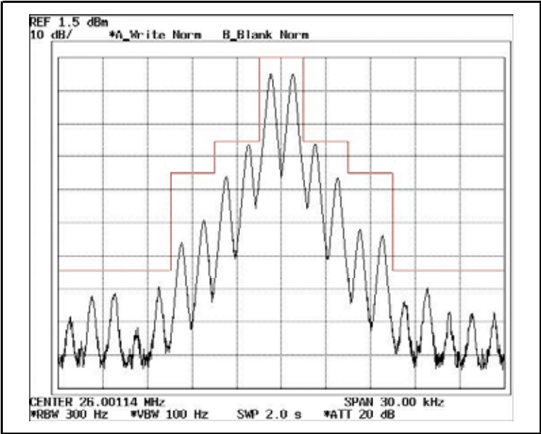
Frequency 26.0 MHz MASK A
