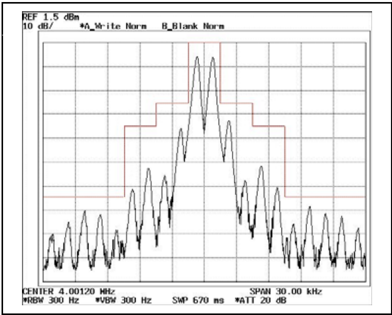
Frequency 4.0 MHz MASK A
