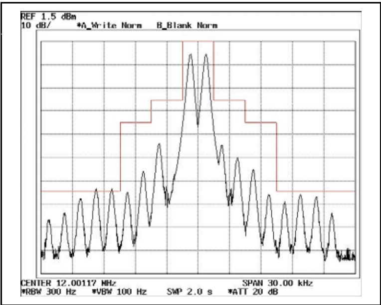
Frequency 12.0 MHz MASK A
