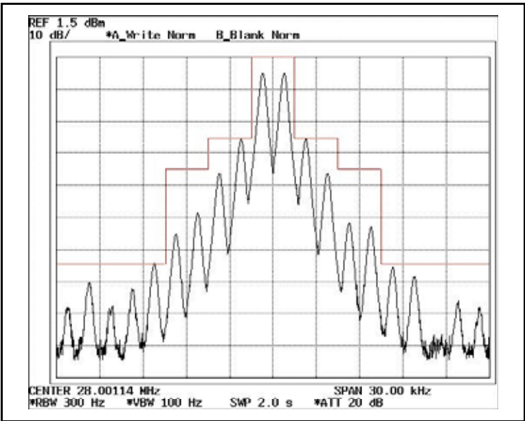
Frequency 28.0 MHz MASK A
