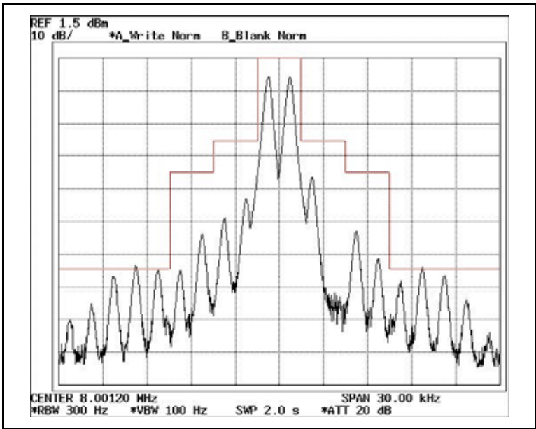
Frequency 8.0 MHz MASK A
