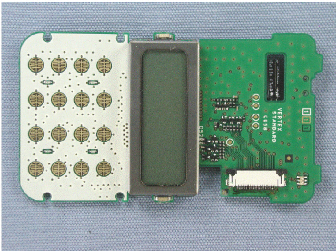
Side-A of DISPLAY-UNIT with LCD (VX-824/829/VX-874/879)
