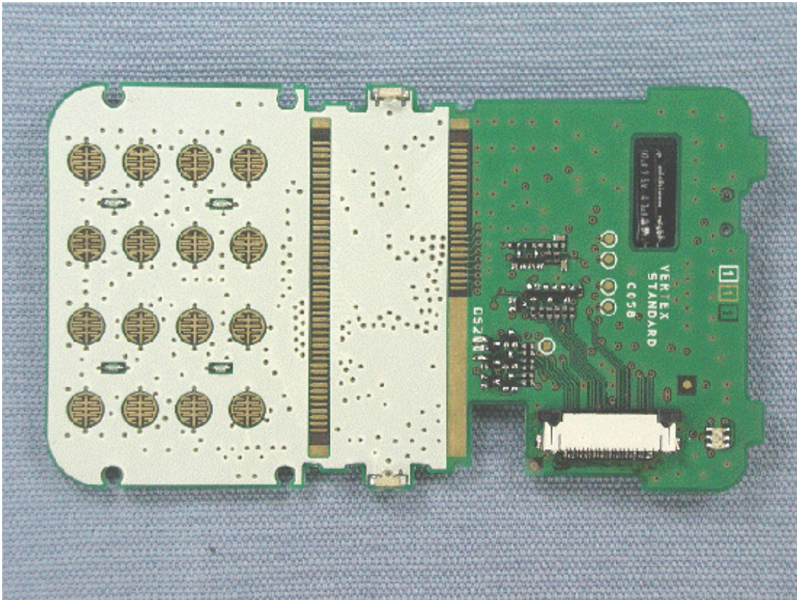
Side-A of DISPLAY-UNIT without LCD (VX-824/829/VX-874/879)
