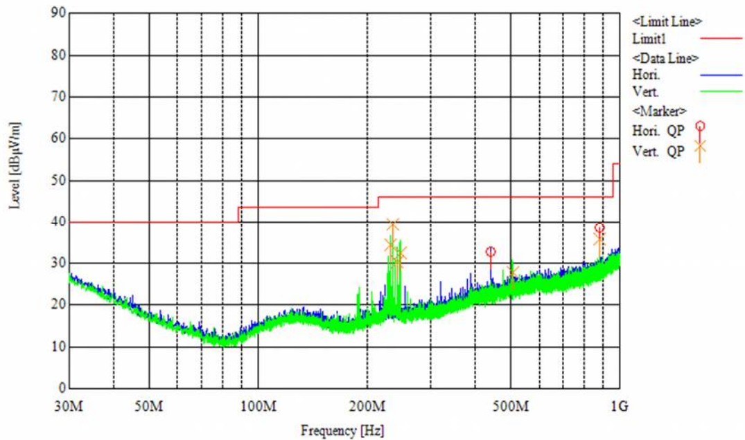
[Chart] Tx 2440MHz DH5
