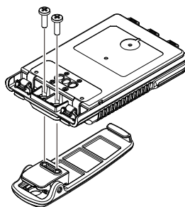
Battery Latches
